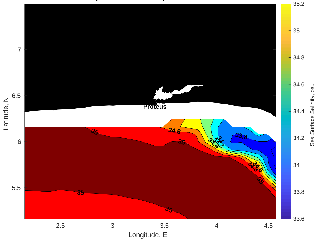
Surface Salinity for Proteus at 21-Apr-2025 00:00:00
