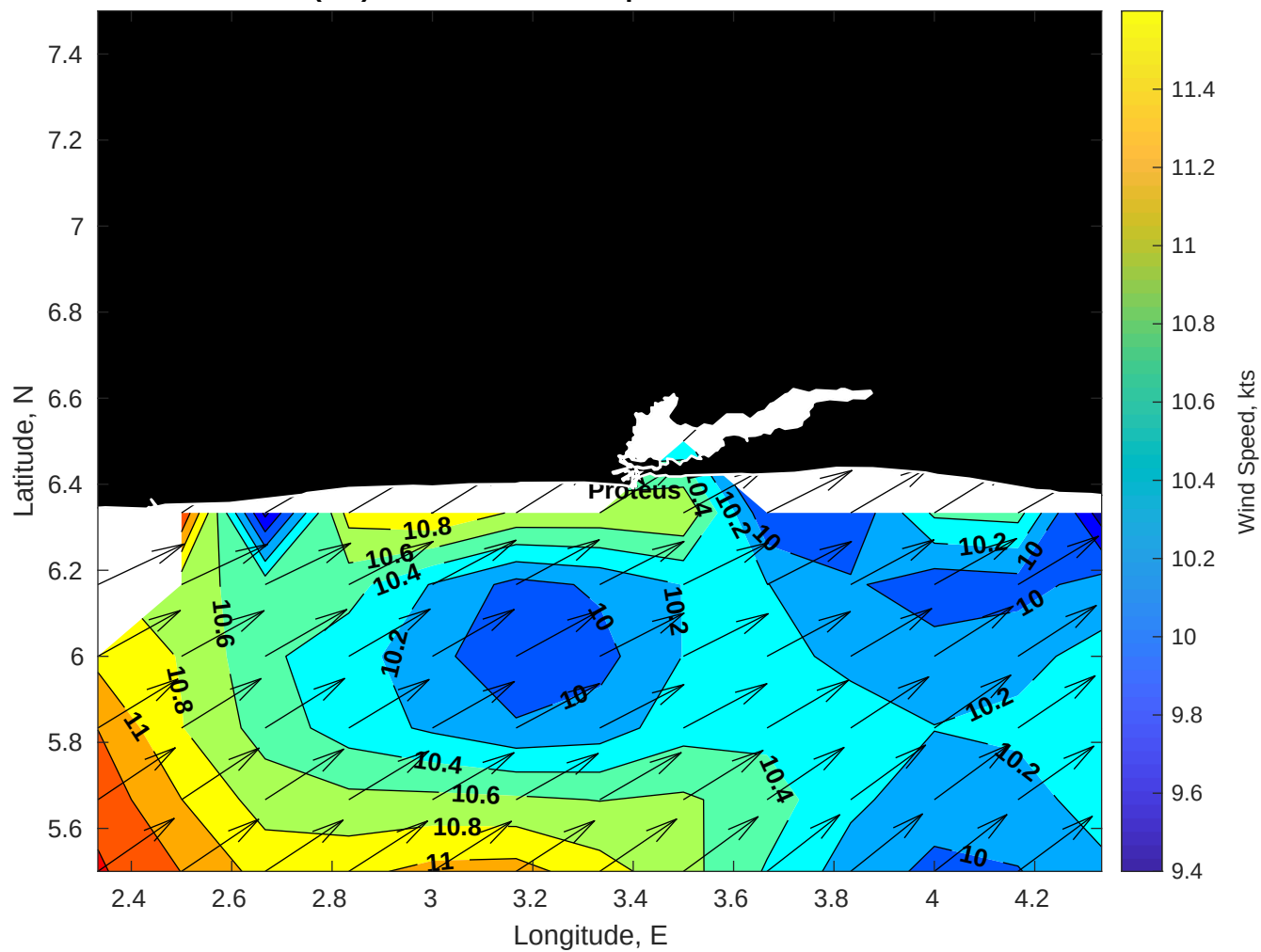
Winds (kts) for Proteus at 22-Apr-2025 09:00:00
