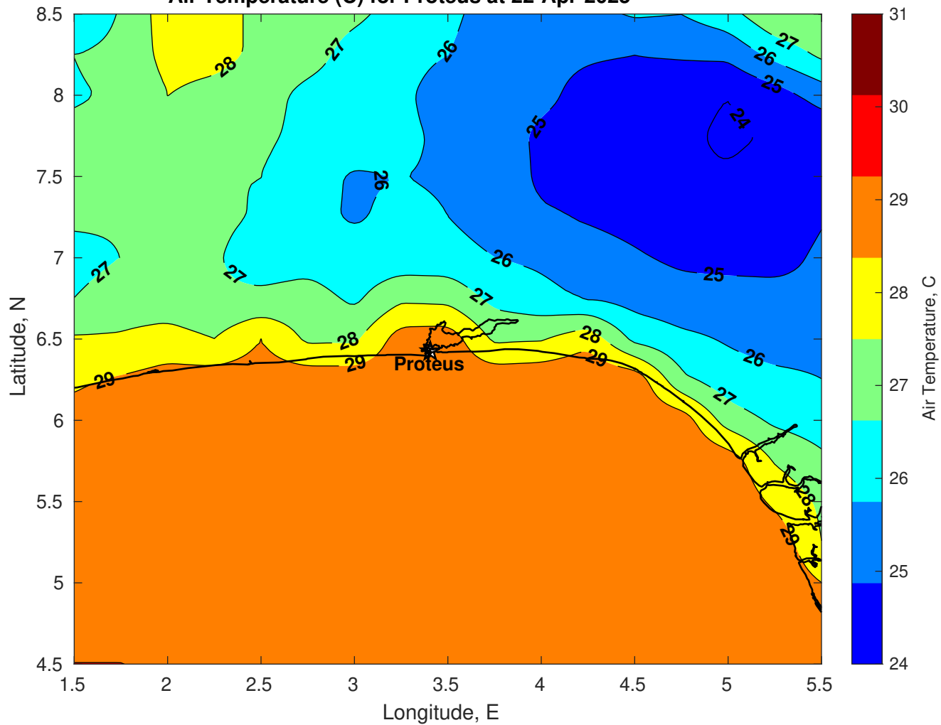
Air Temperature (C) for Proteus at 22-Apr-2025
