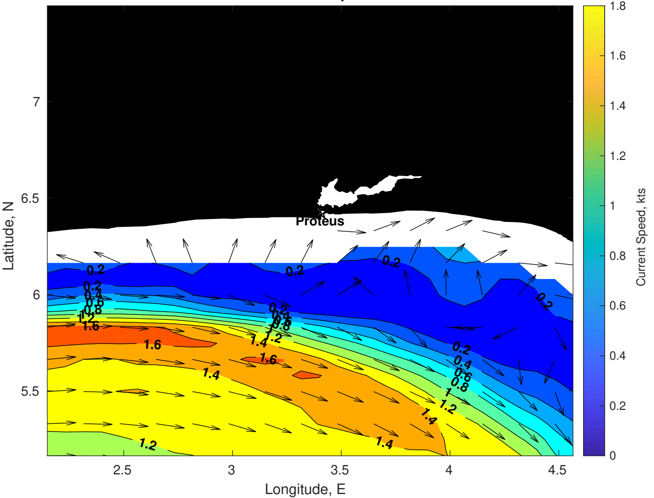
Surface Currents for Proteus at 21-Apr-2025 00:00:00
