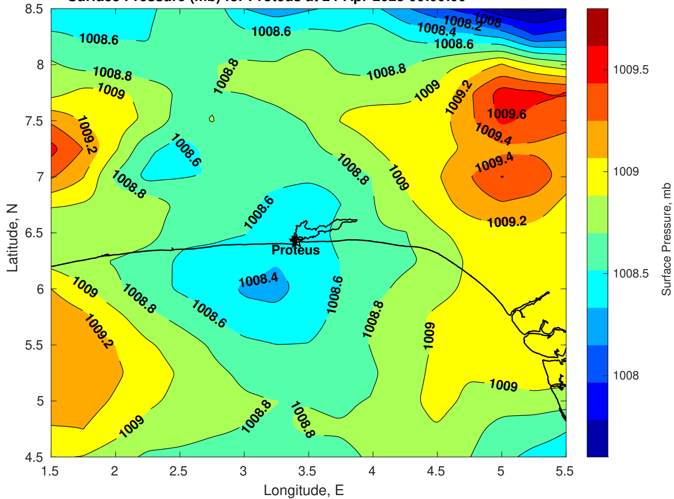
Surface Pressure (mb) for Proteus at 24-Apr-2025 00:00:00
