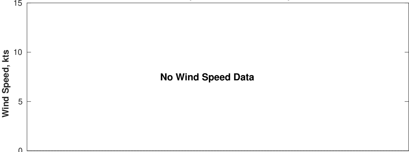
Wind & Wave Forecast for Proteus from 22-Apr-2025 01:00:00 to 08-May-2025 01:00:00
