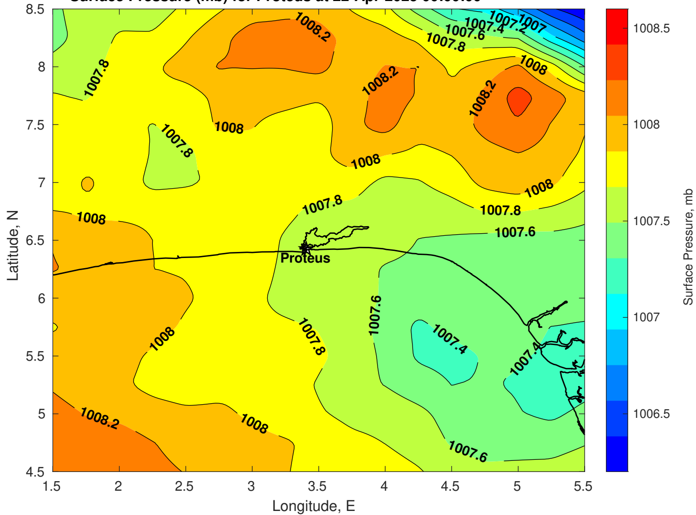
Surface Pressure (mb) for Proteus at 22-Apr-2025 00:00:00
