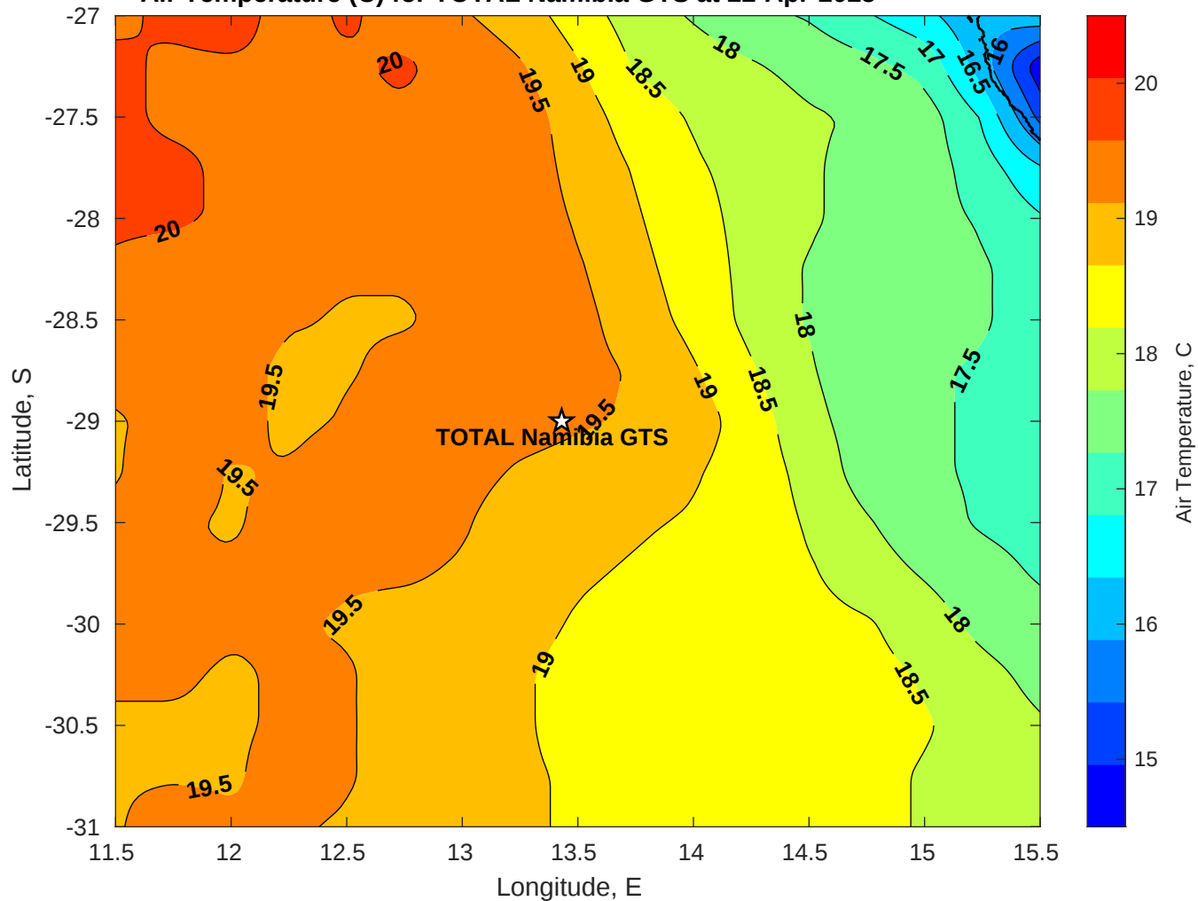
Air Temperature (C) for TOTAL Namibia GTS at 22-Apr-2025
