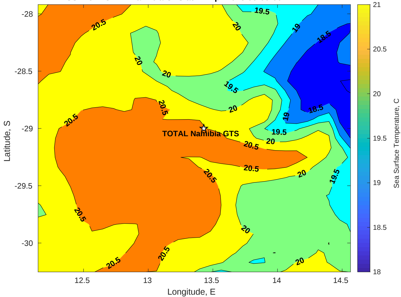
SST for TOTAL Namibia GTS at 21-Apr-2025 00:00:00
