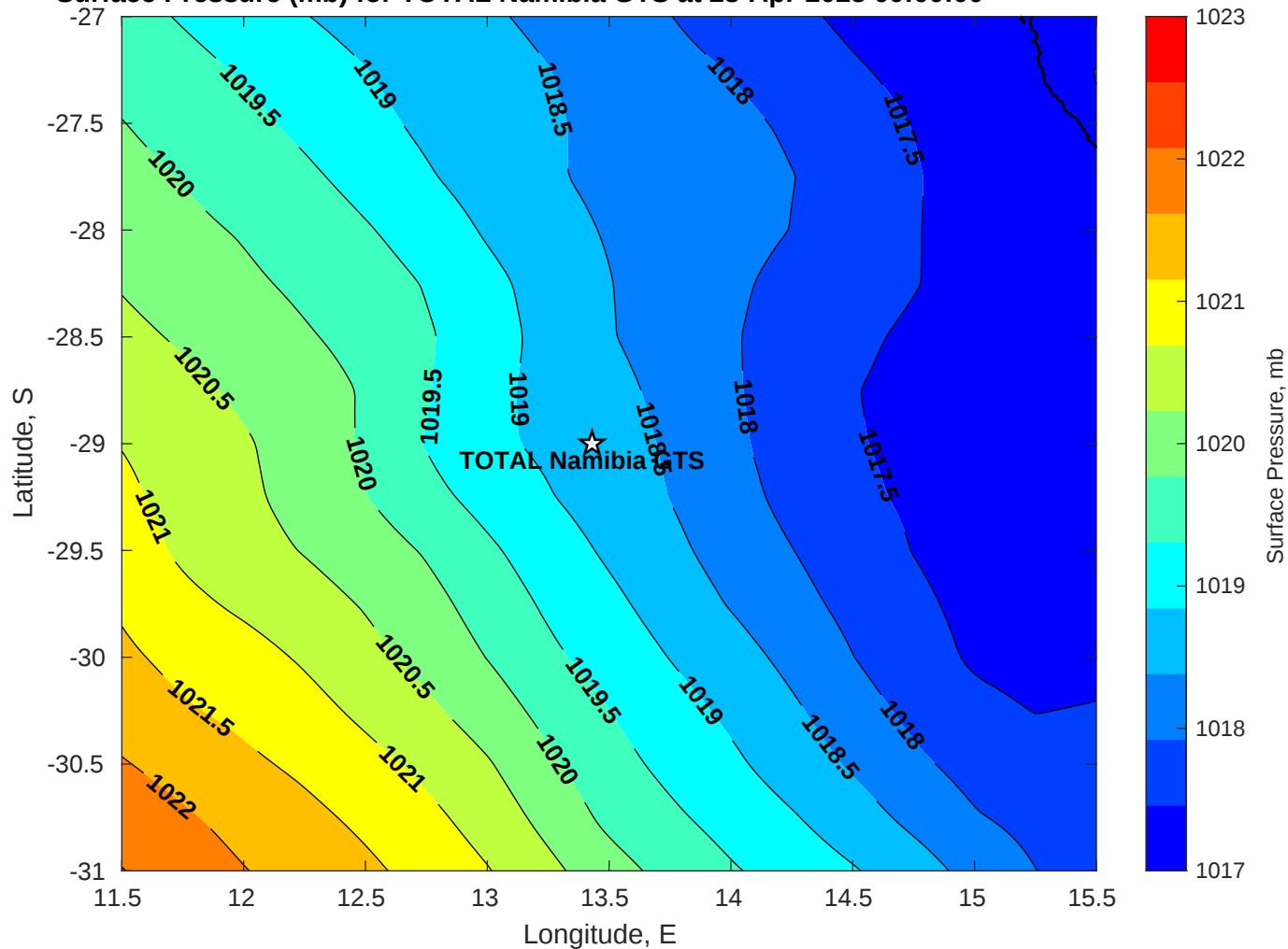
Surface Pressure (mb) for TOTAL Namibia GTS at 23-Apr-2025 00:00:00
