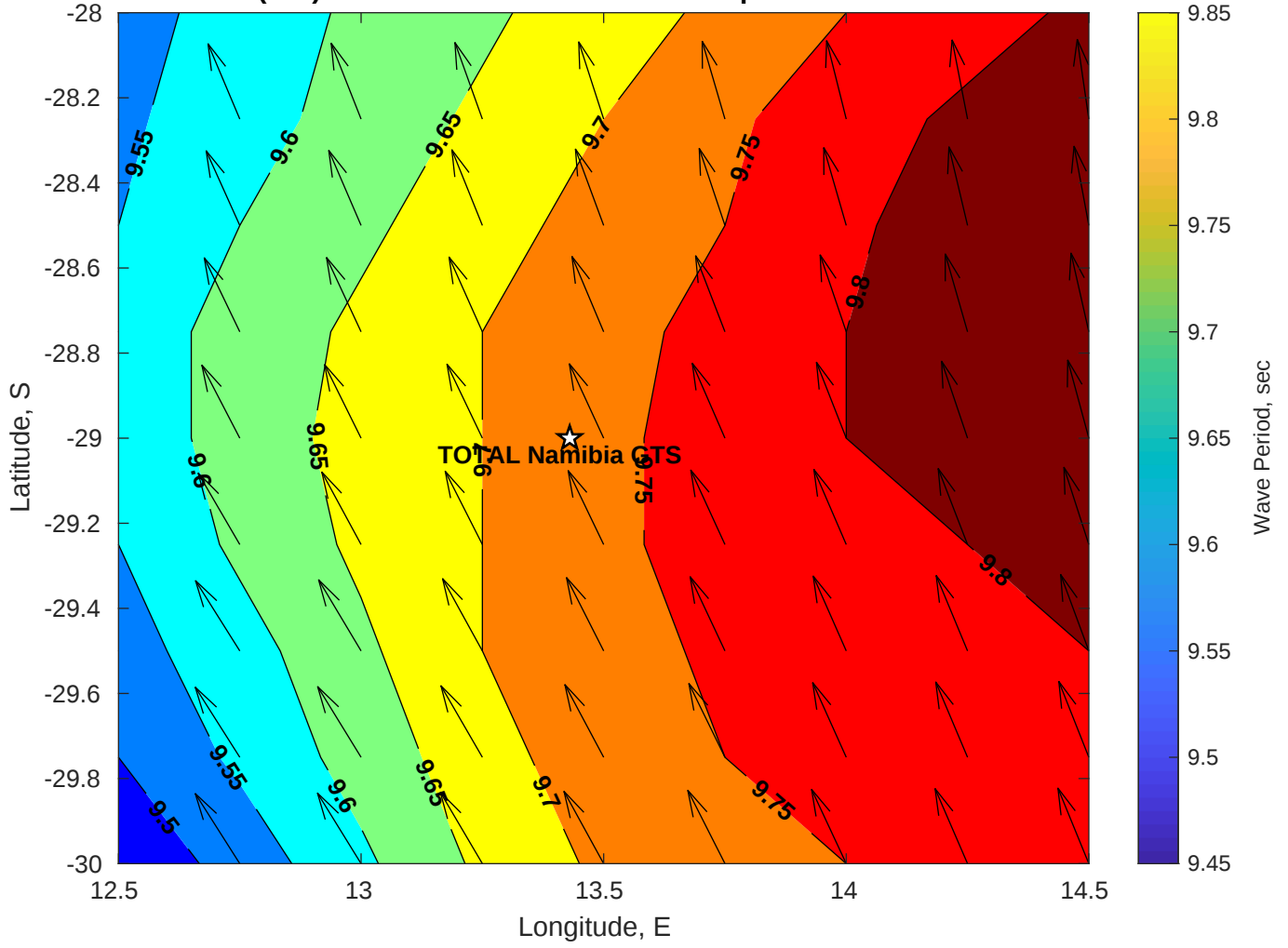
Wave Period (sec) for TOTAL Namibia GTS at 22-Apr-2025 09:00:00
