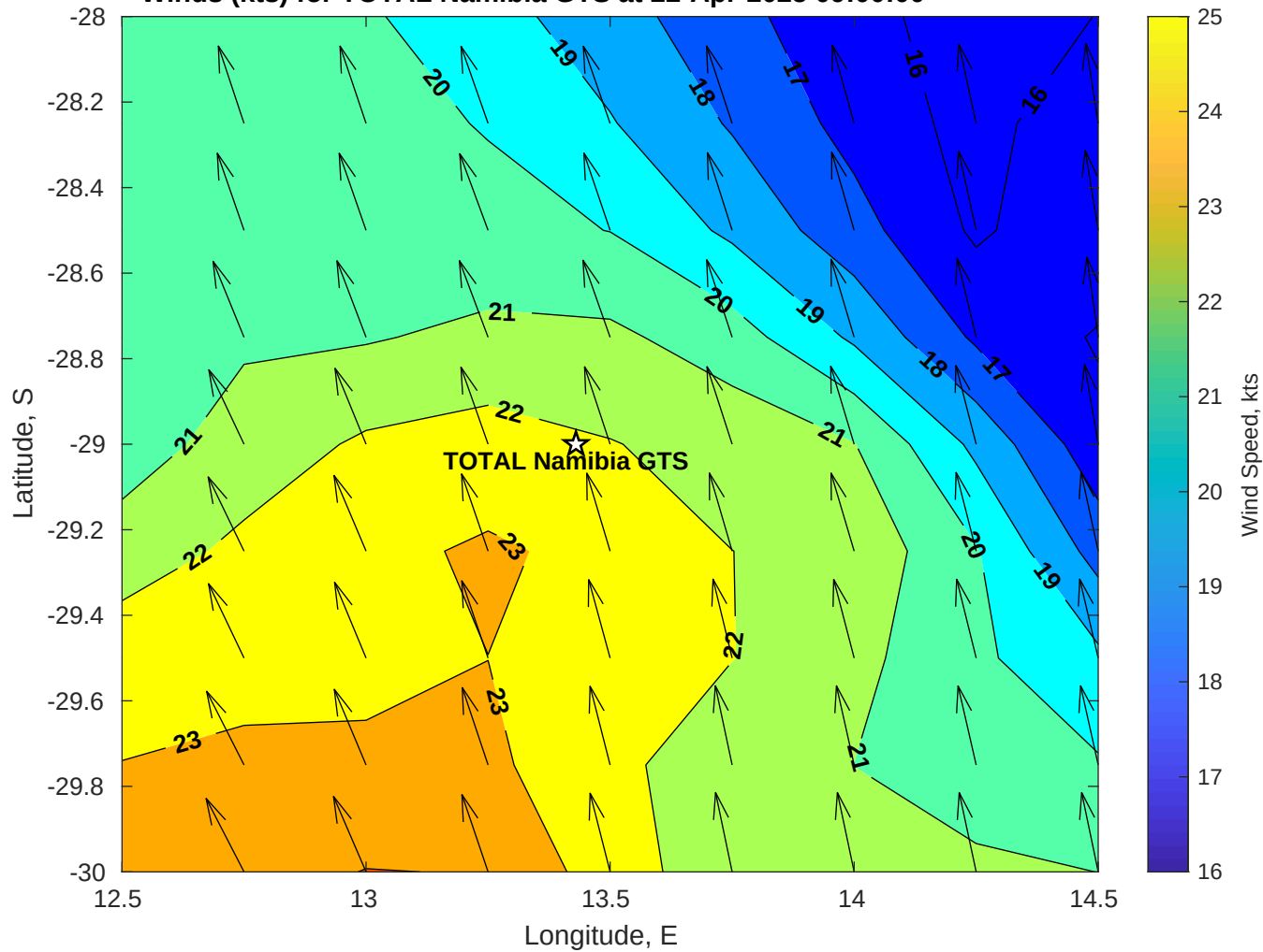
Winds (kts) for TOTAL Namibia GTS at 22-Apr-2025 09:00:00
