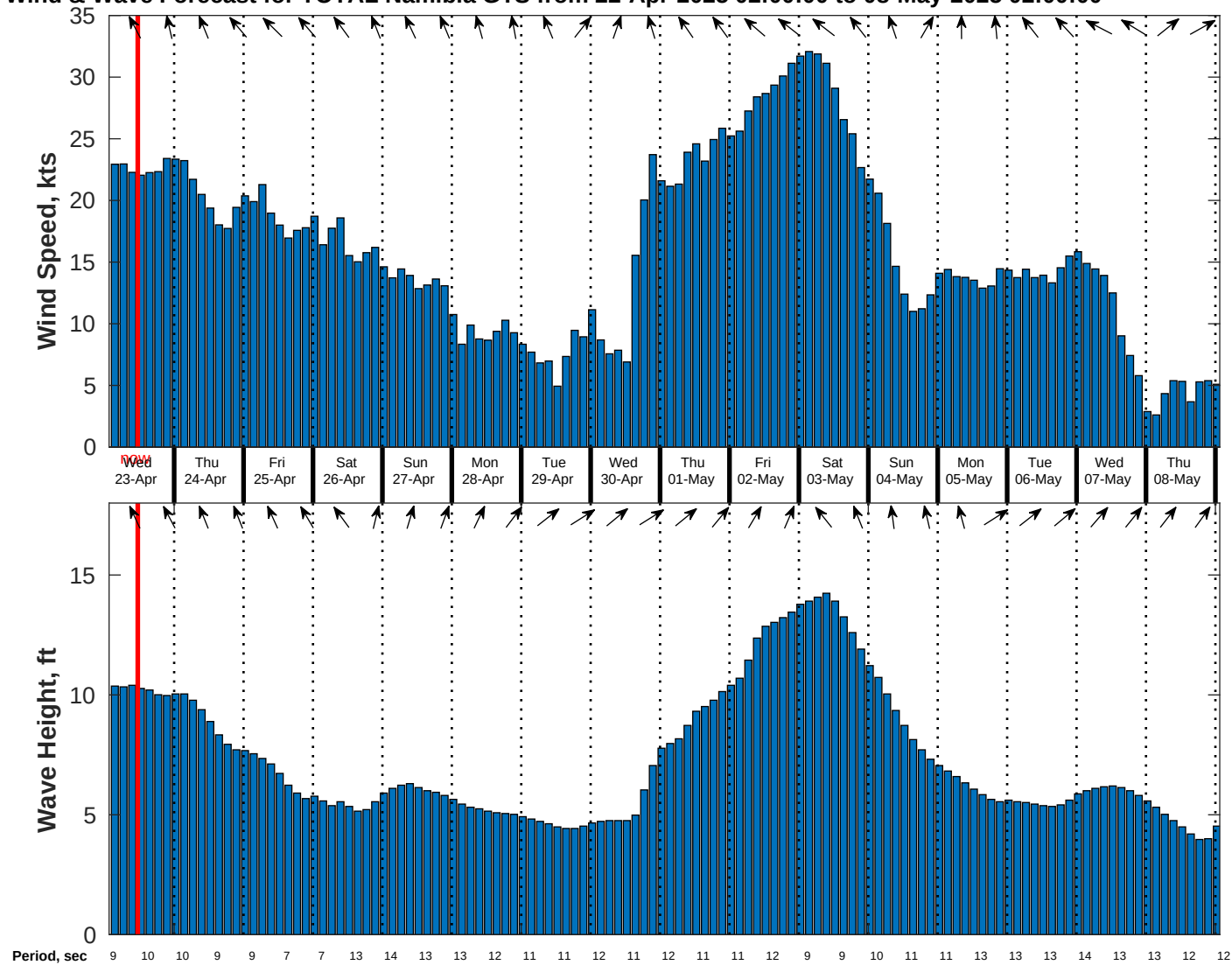
Wind & Wave Forecast for TOTAL Namibia GTS from 22-Apr-2025 02:00:00 to 08-May-2025 02:00:00
