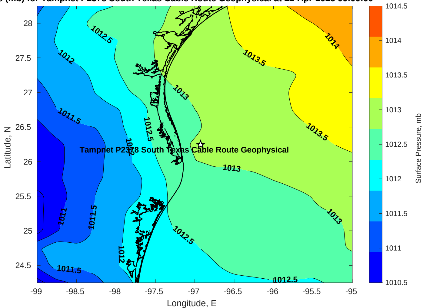
Pressure (mb) for Tampnet P2378 South Texas Cable Route Geophysical at 22-Apr-2025 00:00:00
