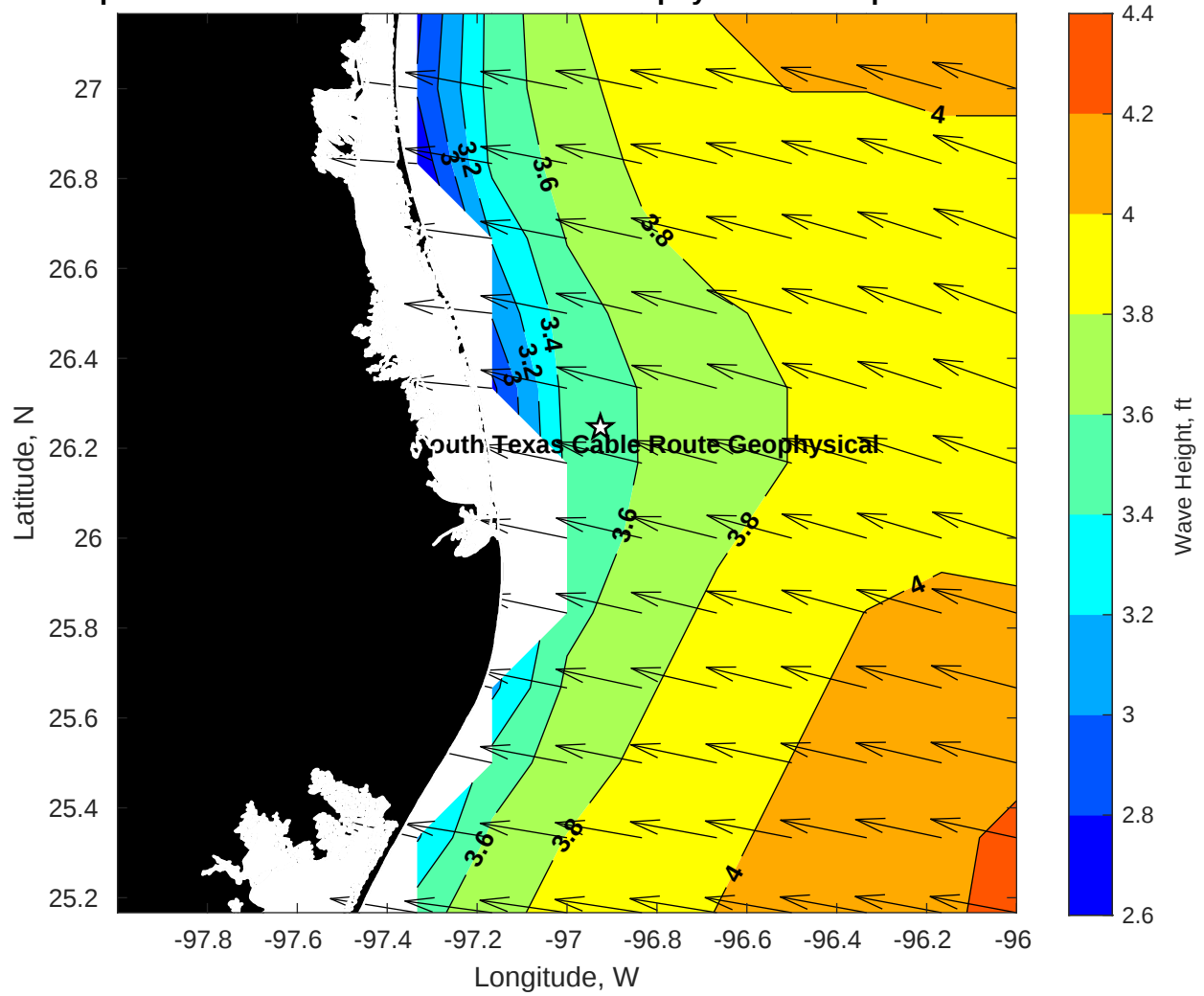
Wave Height (ft) for Tampnet P2378 South Texas Cable Route Geophysical at 22-Apr-2025 09:00:00
