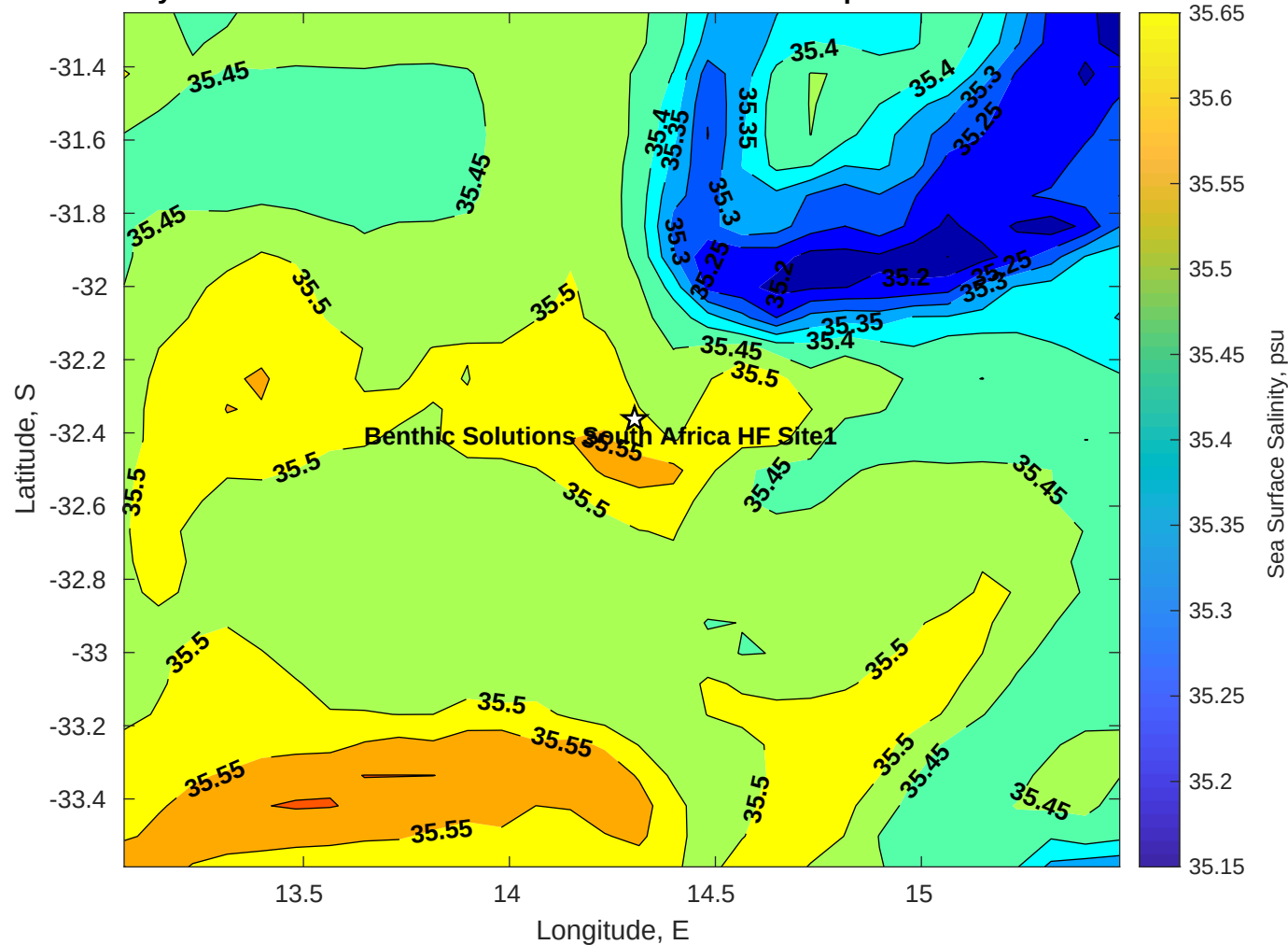
Surface Salinity for Benthic Solutions South Africa HF Site1 at 22-Apr-2025 00:00:00
