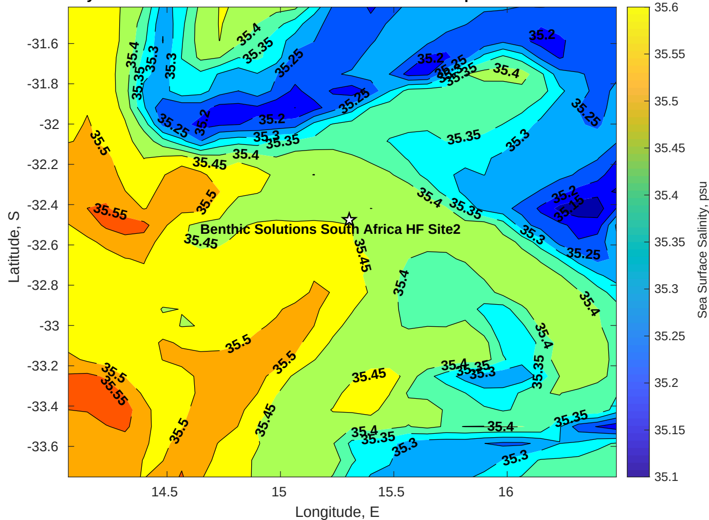
Surface Salinity for Benthic Solutions South Africa HF Site2 at 22-Apr-2025 00:00:00
