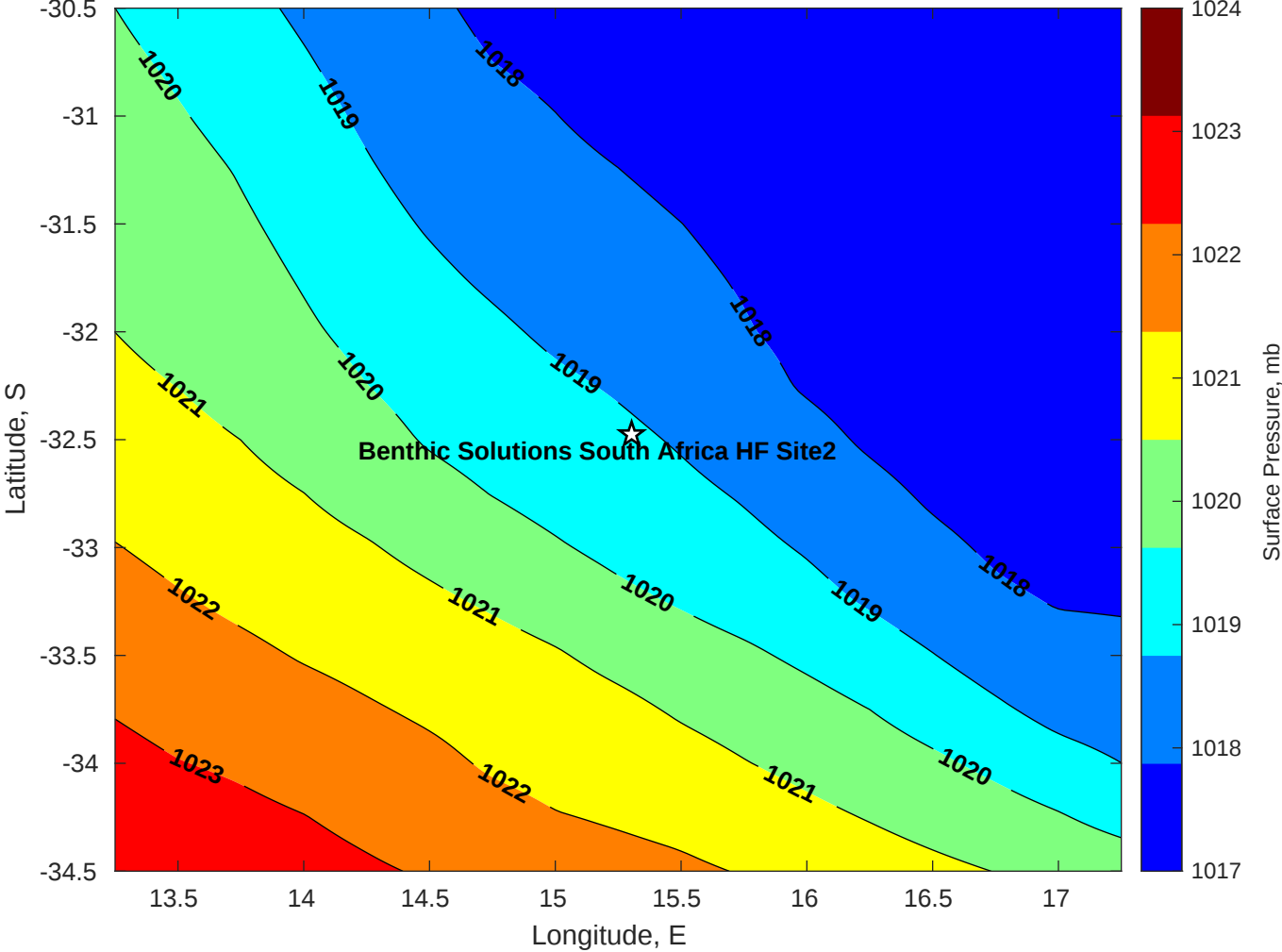
Surface Pressure (mb) for Benthic Solutions South Africa HF Site2 at 23-Apr-2025 00:00:00
