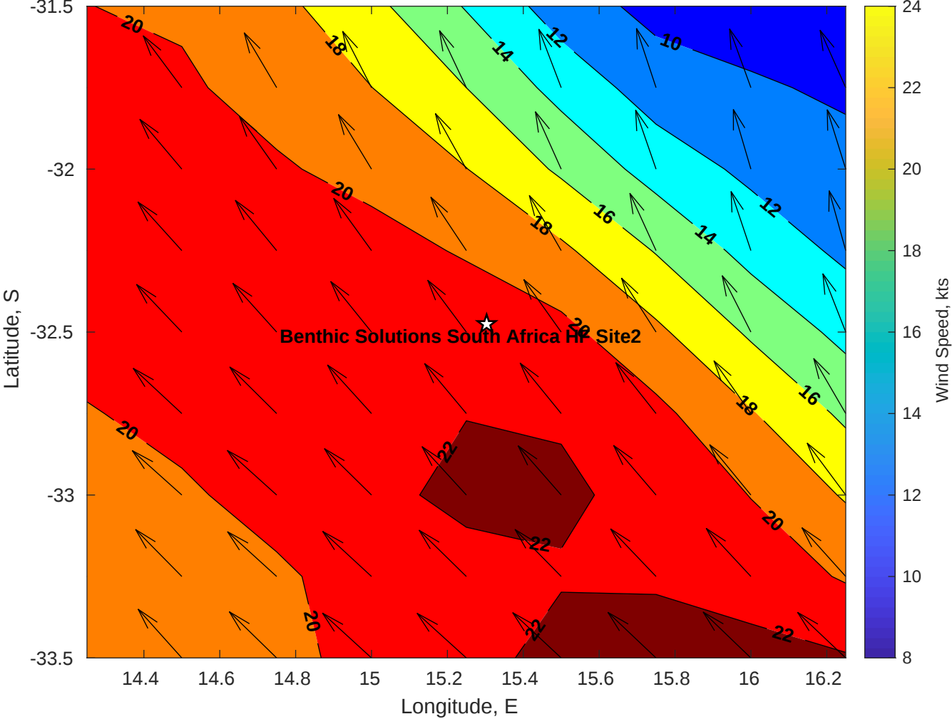
Winds (kts) for Benthic Solutions South Africa HF Site2 at 23-Apr-2025 09:00:00
