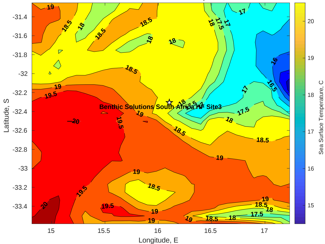
SST for Benthic Solutions South Africa HF Site3 at 22-Apr-2025 00:00:00
