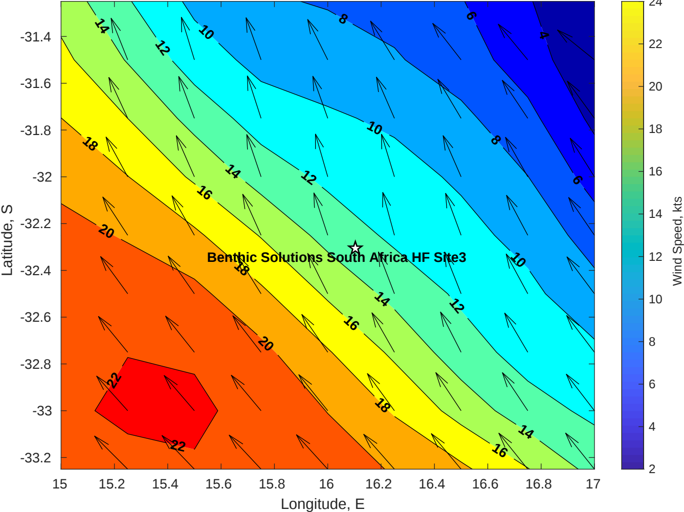
Winds (kts) for Benthic Solutions South Africa HF Site3 at 23-Apr-2025 09:00:00
