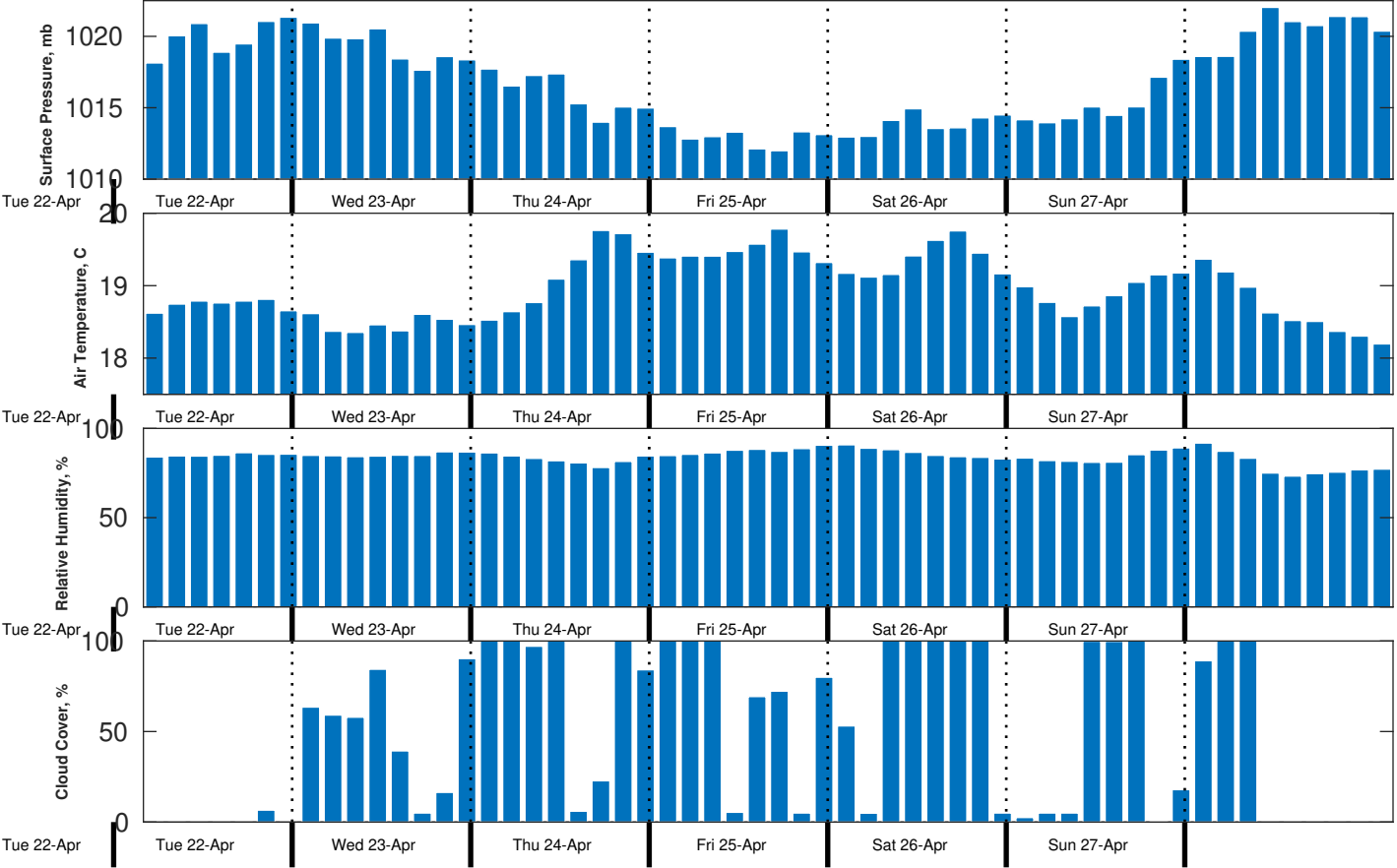
Met Forecast for Benthic Solutions South Africa HF Site3 from 23-Apr-2025 00:00:00 to 30-Apr-2025 00:00:00
