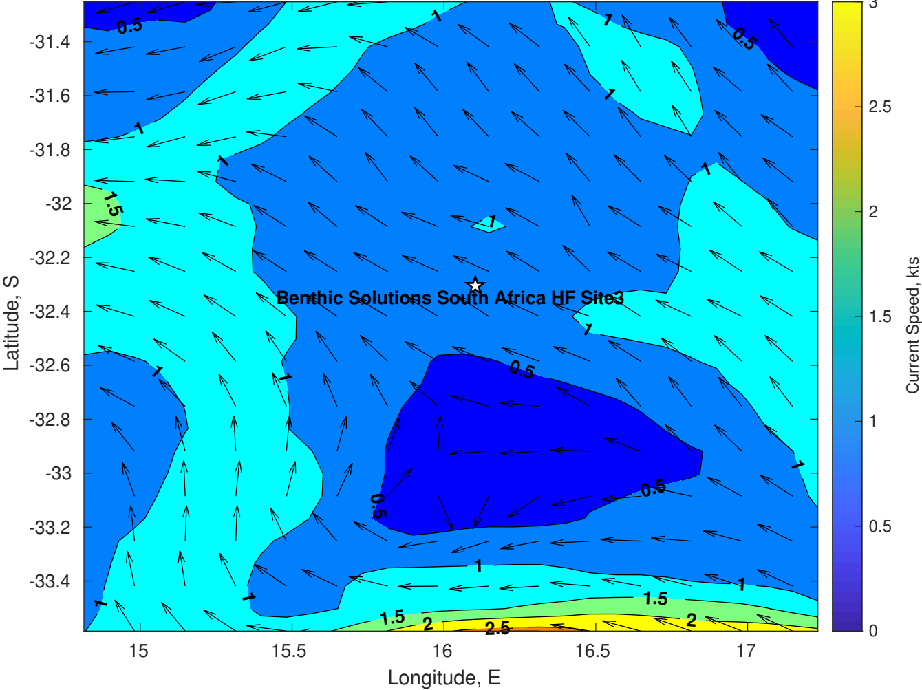
Surface Currents for Benthic Solutions South Africa HF Site3 at 22-Apr-2025 00:00:00
