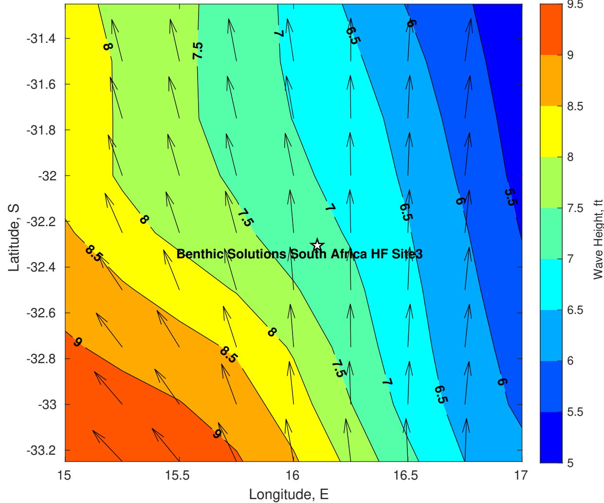
Wave Height (ft) for Benthic Solutions South Africa HF Site3 at 23-Apr-2025 09:00:00
