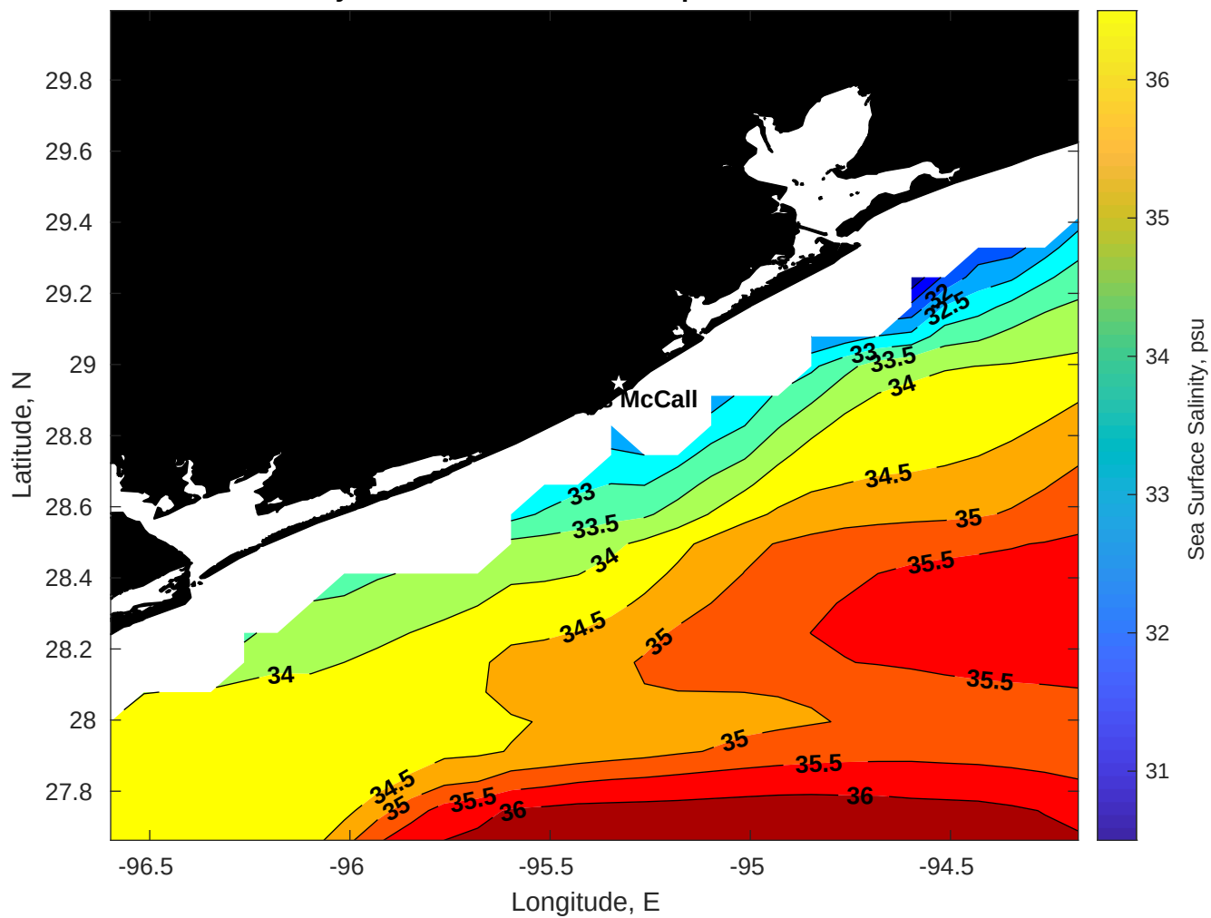
Surface Salinity for Brooks McCall at 22-Apr-2025 00:00:00
