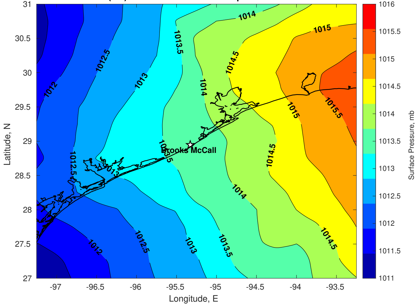
Surface Pressure (mb) for Brooks McCall at 25-Apr-2025 00:00:00
