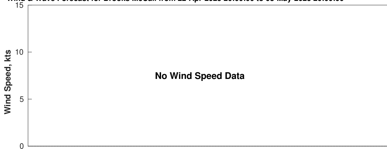
Wind & Wave Forecast for Brooks McCall from 22-Apr-2025 20:00:00 to 08-May-2025 20:00:00
