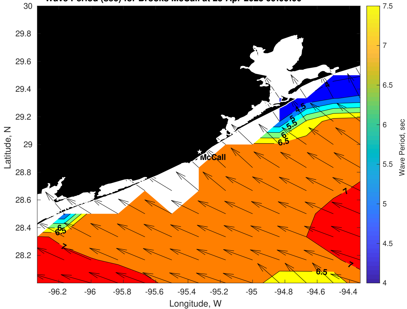
Wave Period (sec) for Brooks McCall at 23-Apr-2025 09:00:00
