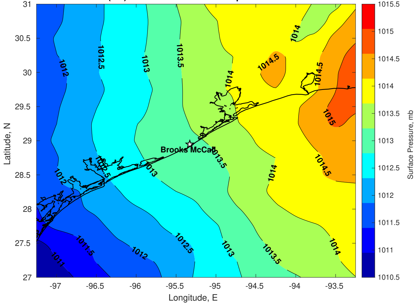
Surface Pressure (mb) for Brooks McCall at 24-Apr-2025 00:00:00
