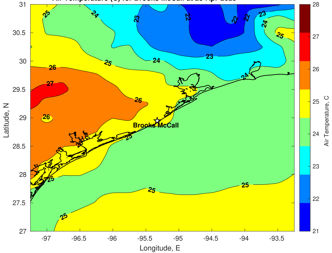
Air Temperature (C) for Brooks McCall at 23-Apr-2025
