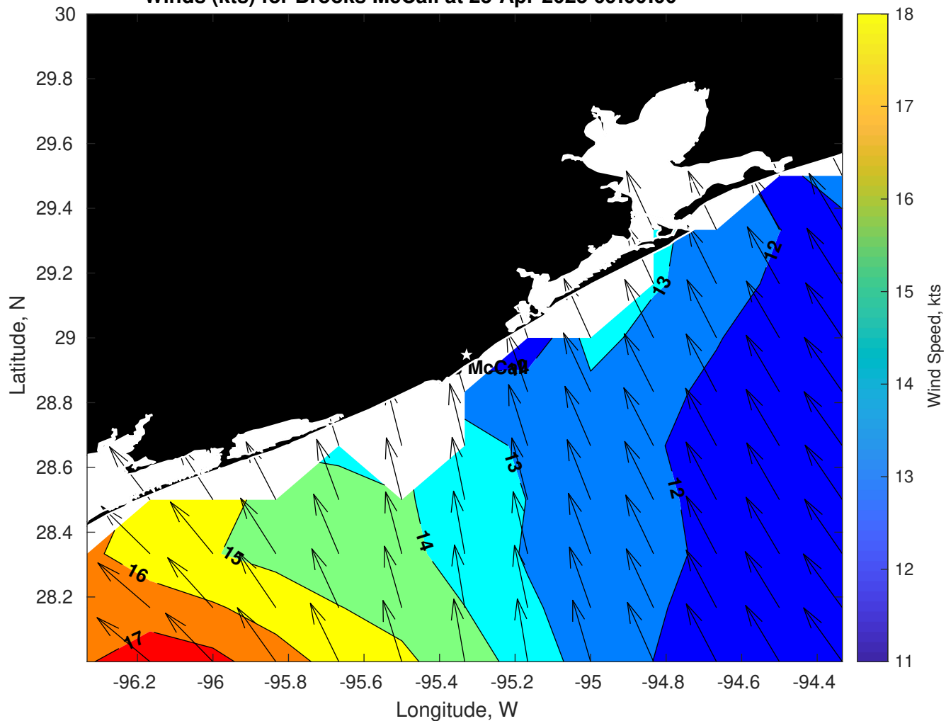
Winds (kts) for Brooks McCall at 23-Apr-2025 09:00:00
