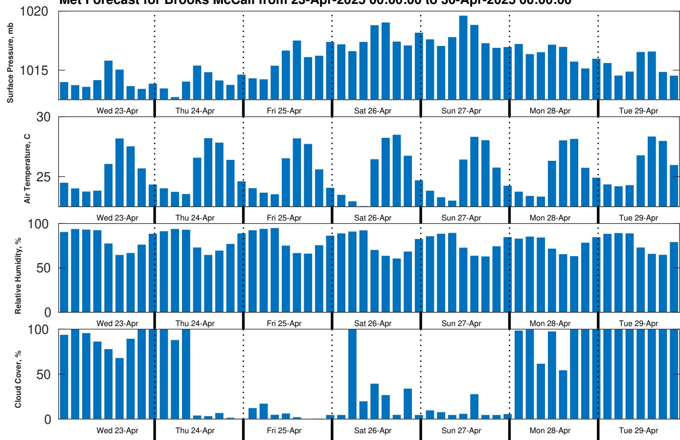
Met Forecast for Brooks McCall from 23-Apr-2025 00:00:00 to 30-Apr-2025 00:00:00
