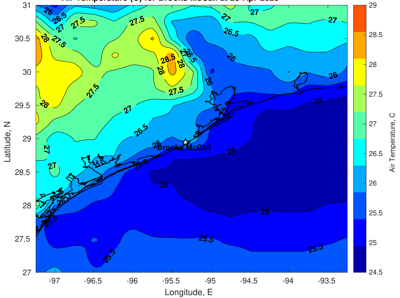
Air Temperature (C) for Brooks McCall at 23-Apr-2025
