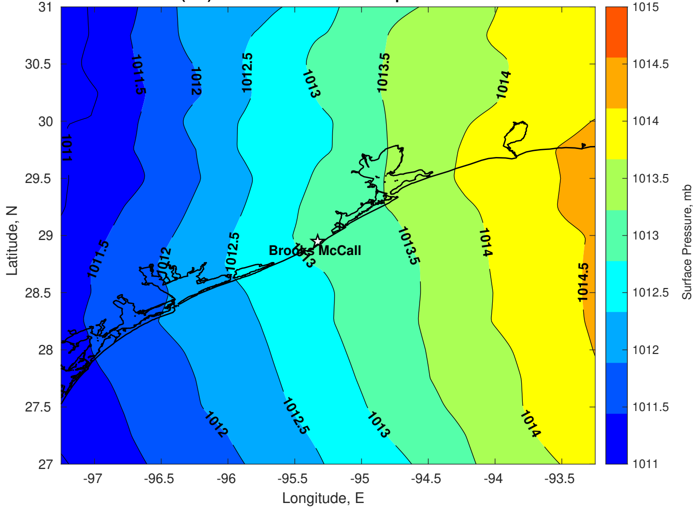
Surface Pressure (mb) for Brooks McCall at 23-Apr-2025 00:00:00
