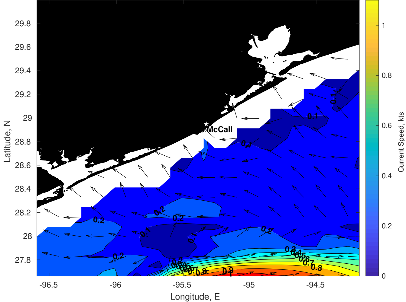
Surface Currents for Brooks McCall at 22-Apr-2025 00:00:00
