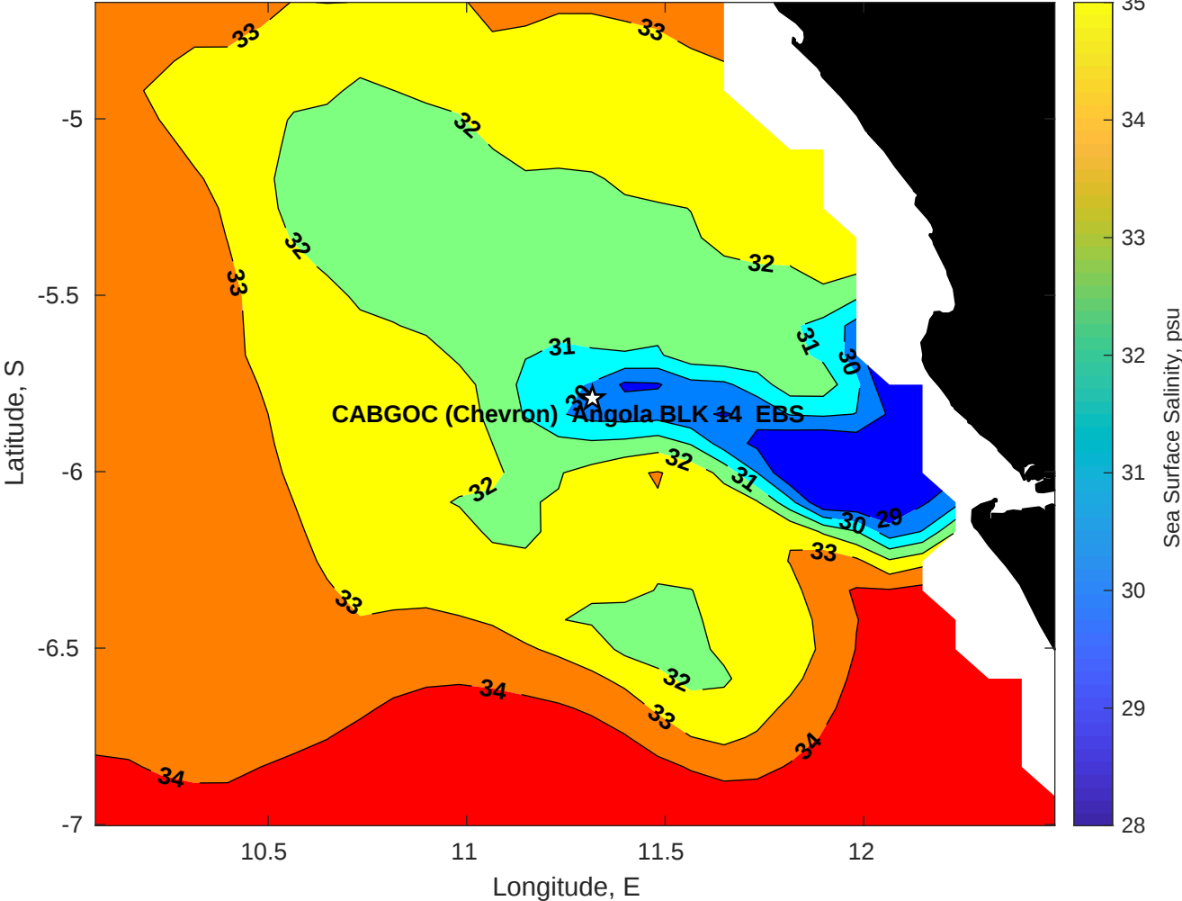
Surface Salinity for CABGOC (Chevron) Angola BLK 14 EBS at 22-Apr-2025 00:00:00
