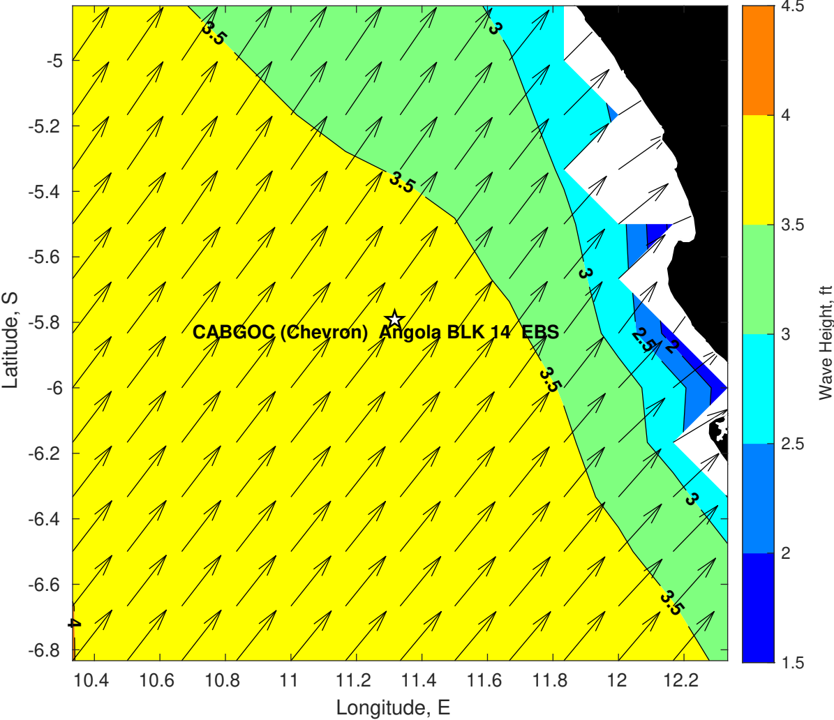
Wave Height (ft) for CABGOC (Chevron) Angola BLK 14 EBS at 23-Apr-2025 09:00:00
