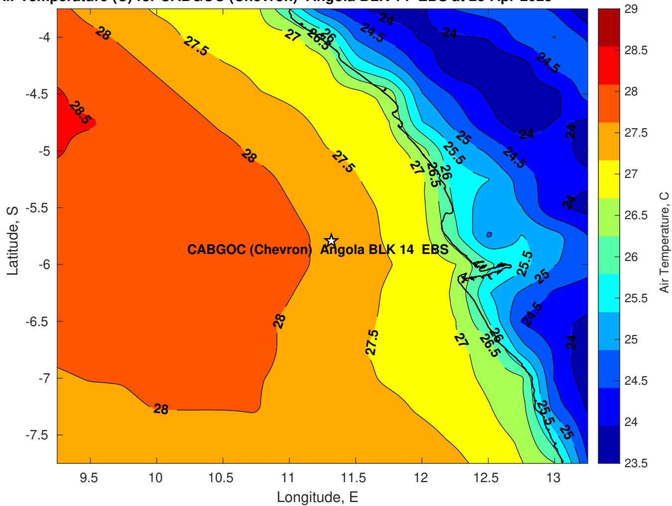
Air Temperature (C) for CABGOC (Chevron) Angola BLK 14 EBS at 23-Apr-2025
