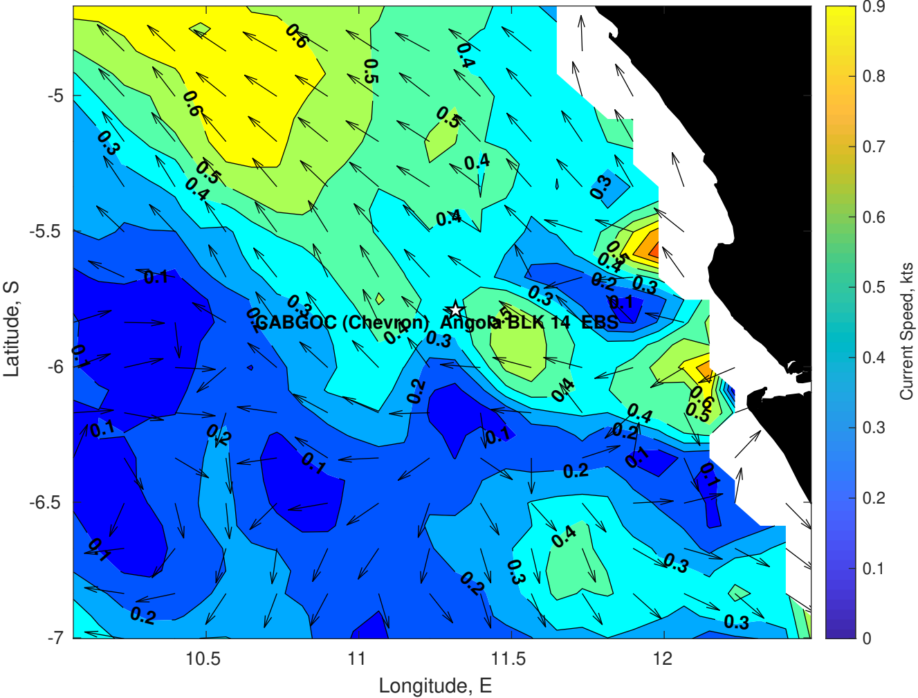
Surface Currents for CABGOC (Chevron) Angola BLK 14 EBS at 22-Apr-2025 00:00:00
