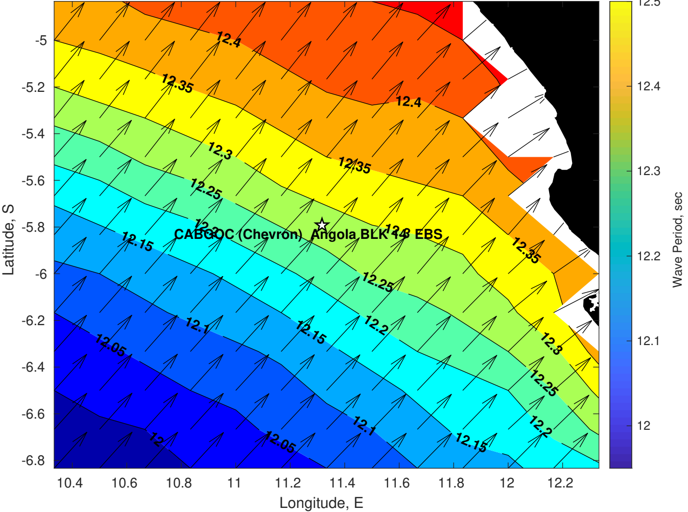
Wave Period (sec) for CABGOC (Chevron) Angola BLK 14 EBS at 23-Apr-2025 09:00:00
