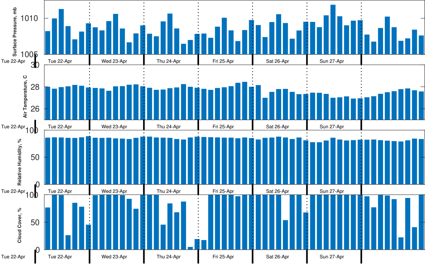
Met Forecast for CABGOC (Chevron) Angola BLK 14 EBS from 23-Apr-2025 00:00:00 to 30-Apr-2025 00:00:00
