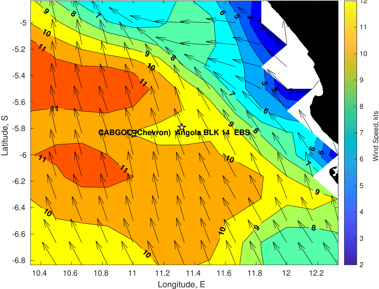
Winds (kts) for CABGOC (Chevron) Angola BLK 14 EBS at 23-Apr-2025 09:00:00
