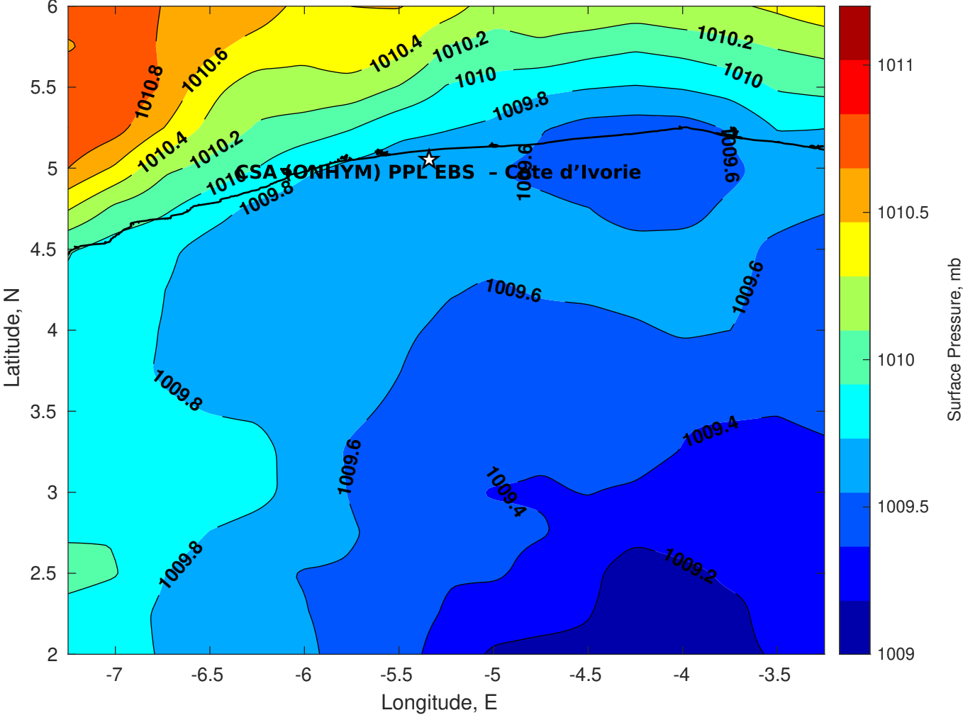
Surface Pressure (mb) for CSA (ONHYM) PPL EBS - Cote d'Ivoire at 24-Apr-2025 00:00:00
