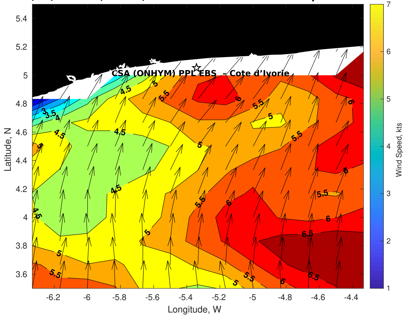
Winds (kts) for CSA (ONHYM) PPL EBS - Cote d'Ivoire at 23-Apr-2025 09:00:00
