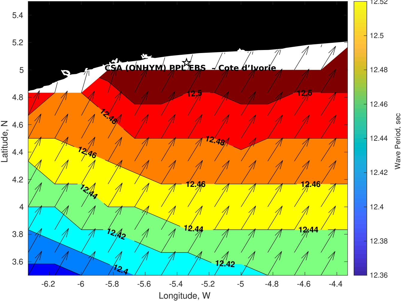
Wave Period (sec) for CSA (ONHYM) PPL EBS - Cote d'Ivoire at 23-Apr-2025 09:00:00
