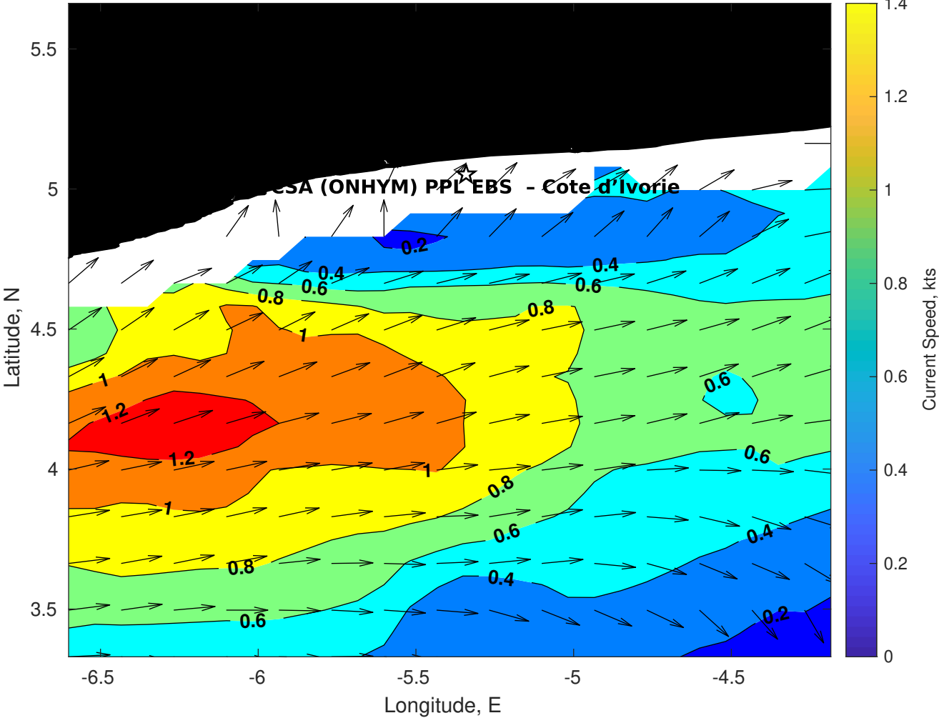
Surface Currents for CSA (ONHYM) PPL EBS - Cote d'Ivoire at 22-Apr-2025 00:00:00
