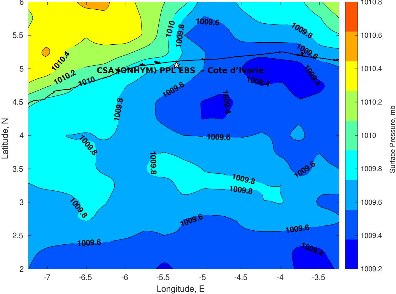
Surface Pressure (mb) for CSA (ONHYM) PPL EBS - Cote d'Ivoire at 23-Apr-2025 00:00:00
