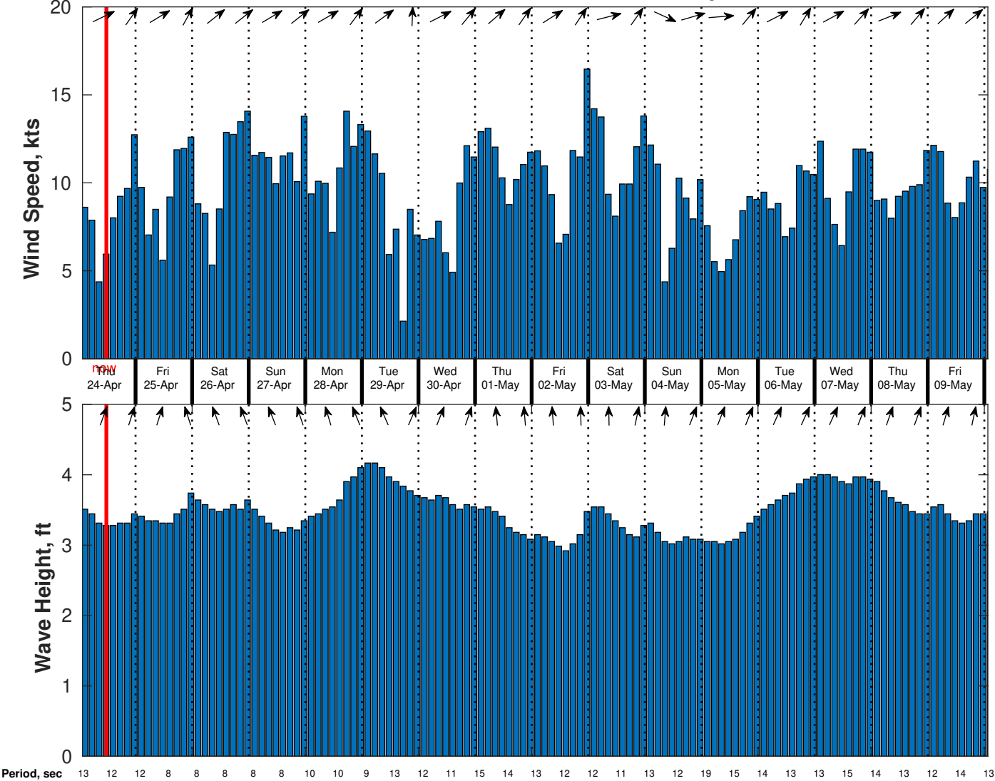
Wind & Wave Forecast for CSA (ONHYM) PPL EBS - Cote d'Ivoire from 23-Apr-2025 01:00:00 to 09-May-2025 01:00:00
