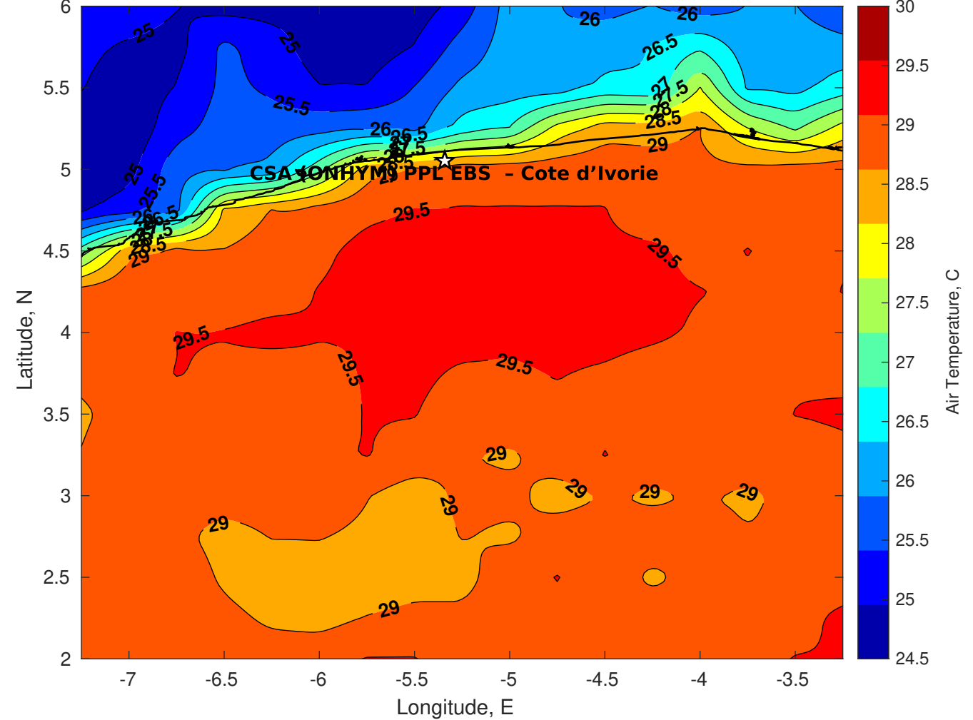
Air Temperature (C) for CSA (ONHYM) PPL EBS - Cote d'Ivoire at 23-Apr-2025
