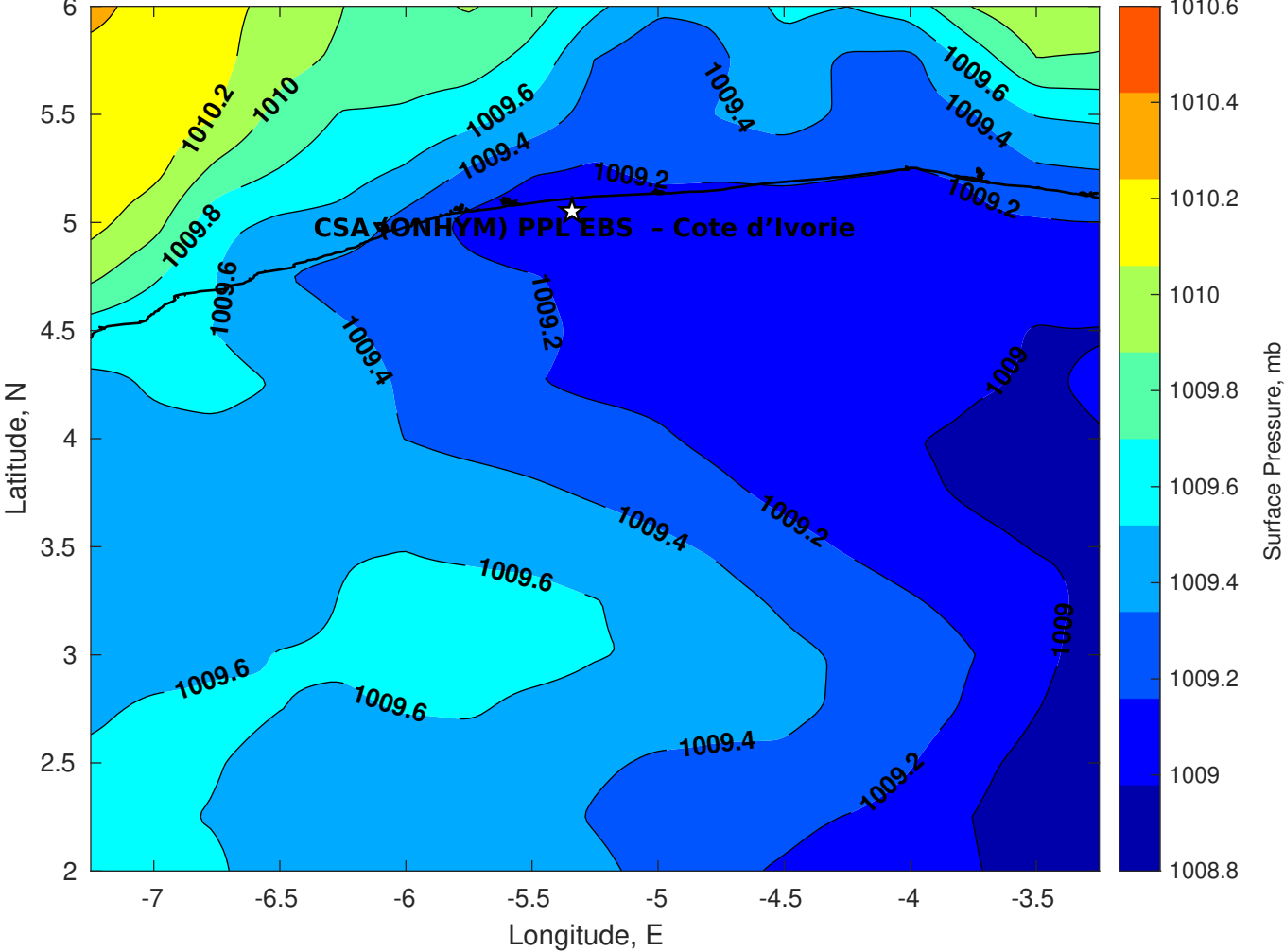
Surface Pressure (mb) for CSA (ONHYM) PPL EBS - Cote d'Ivoire at 25-Apr-2025 00:00:00
