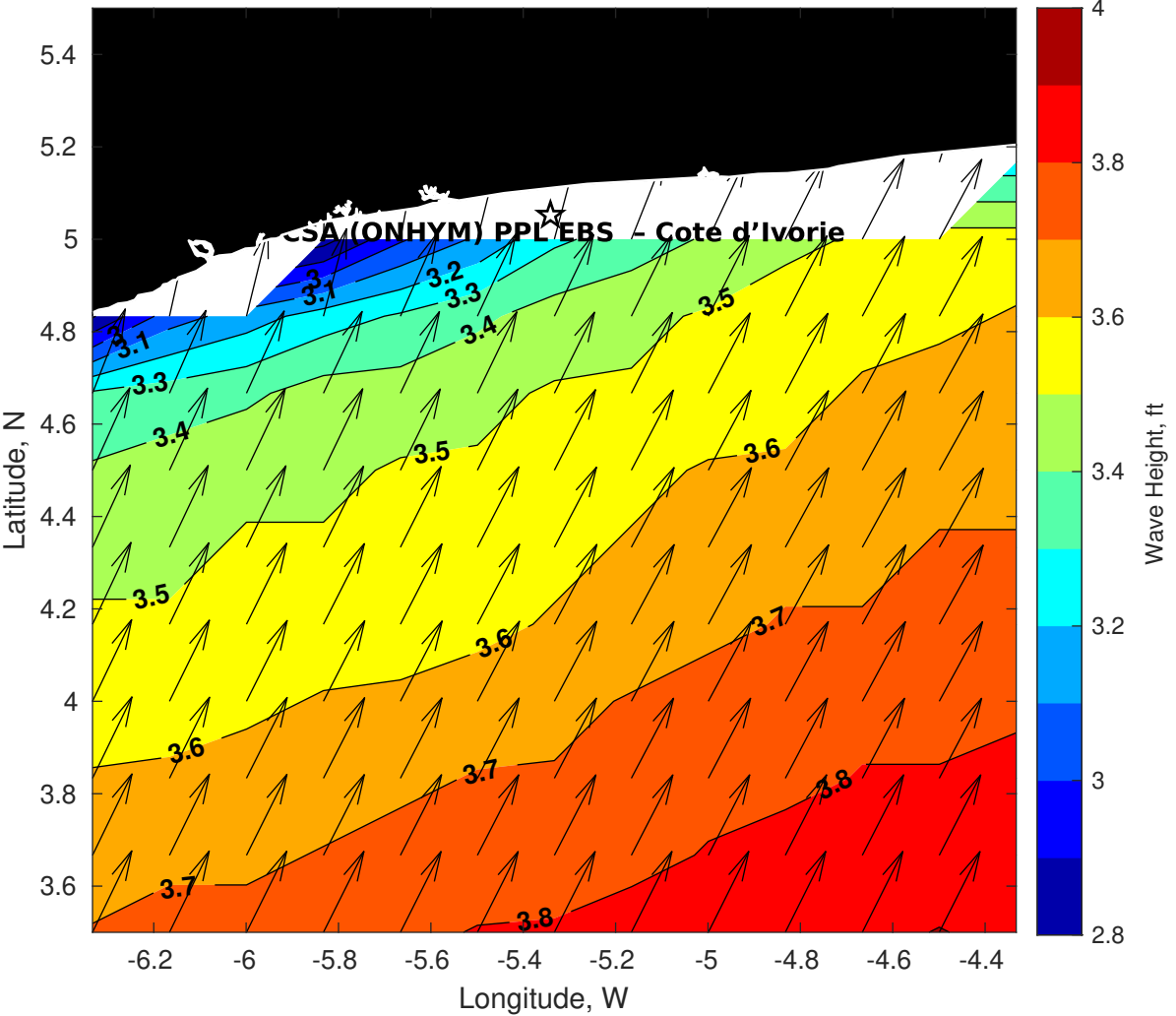
Wave Height (ft) for CSA (ONHYM) PPL EBS - Cote d'Ivoire at 23-Apr-2025 09:00:00
