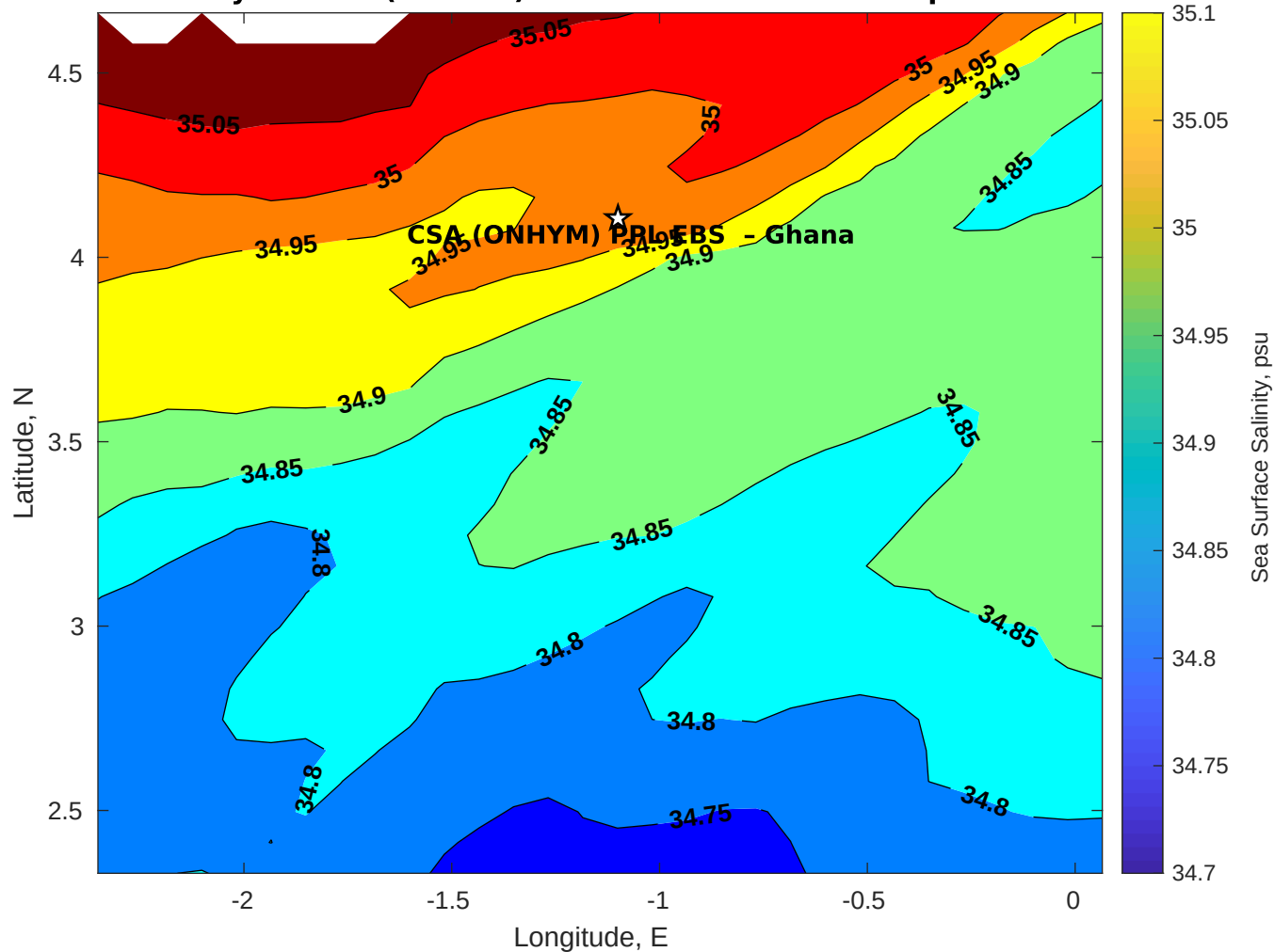
Surface Salinity for CSA (ONHYM) PPL EBS - Ghana at 22-Apr-2025 00:00:00
