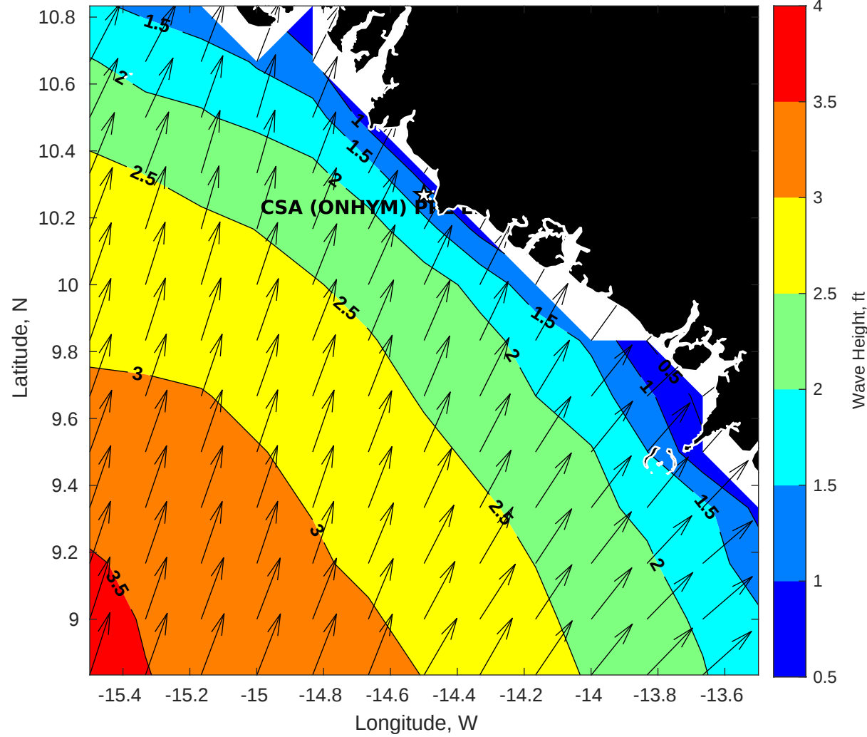
Wave Height (ft) for CSA (ONHYM) PPL EBS - Guinea at 23-Apr-2025 09:00:00
