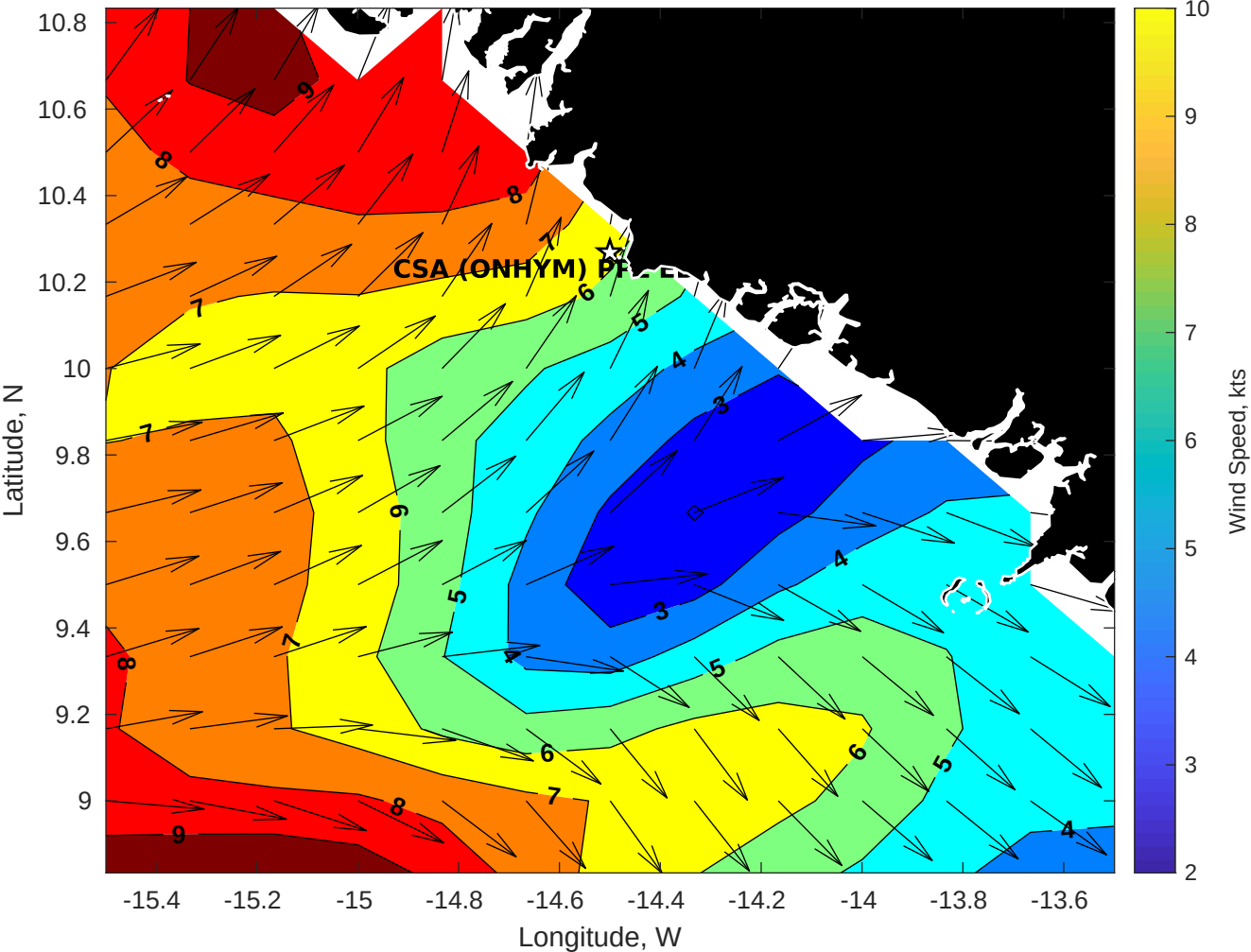
Winds (kts) for CSA (ONHYM) PPL EBS - Guinea at 23-Apr-2025 09:00:00
