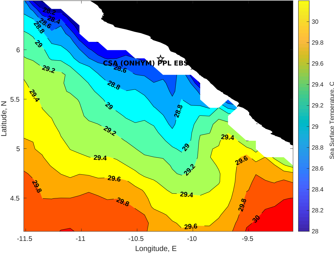
SST for CSA (ONHYM) PPL EBS - Liberia at 22-Apr-2025 00:00:00
