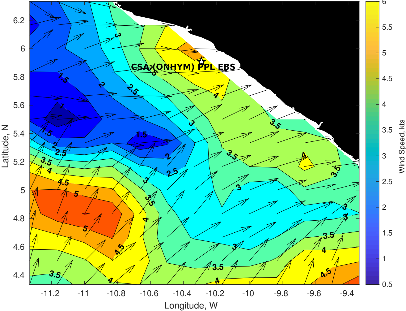
Winds (kts) for CSA (ONHYM) PPL EBS - Liberia at 23-Apr-2025 09:00:00
