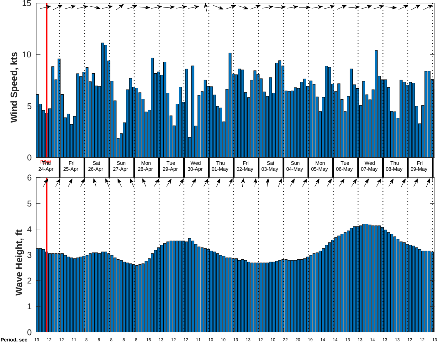
Wind & Wave Forecast for CSA (ONHYM) PPL EBS - Liberia from 23-Apr-2025 01:00:00 to 09-May-2025 01:00:00
