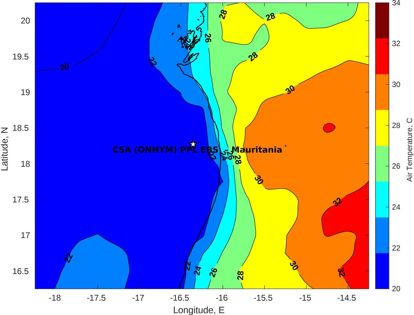
Air Temperature (C) for CSA (ONHYM) PPL EBS - Mauritania at 23-Apr-2025
