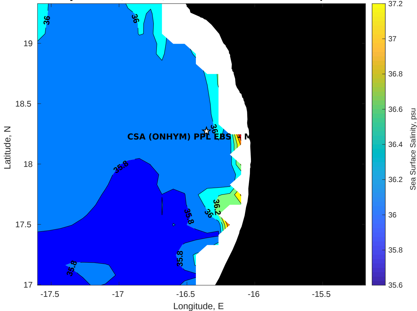
Surface Salinity for CSA (ONHYM) PPL EBS - Mauritania at 22-Apr-2025 00:00:00
