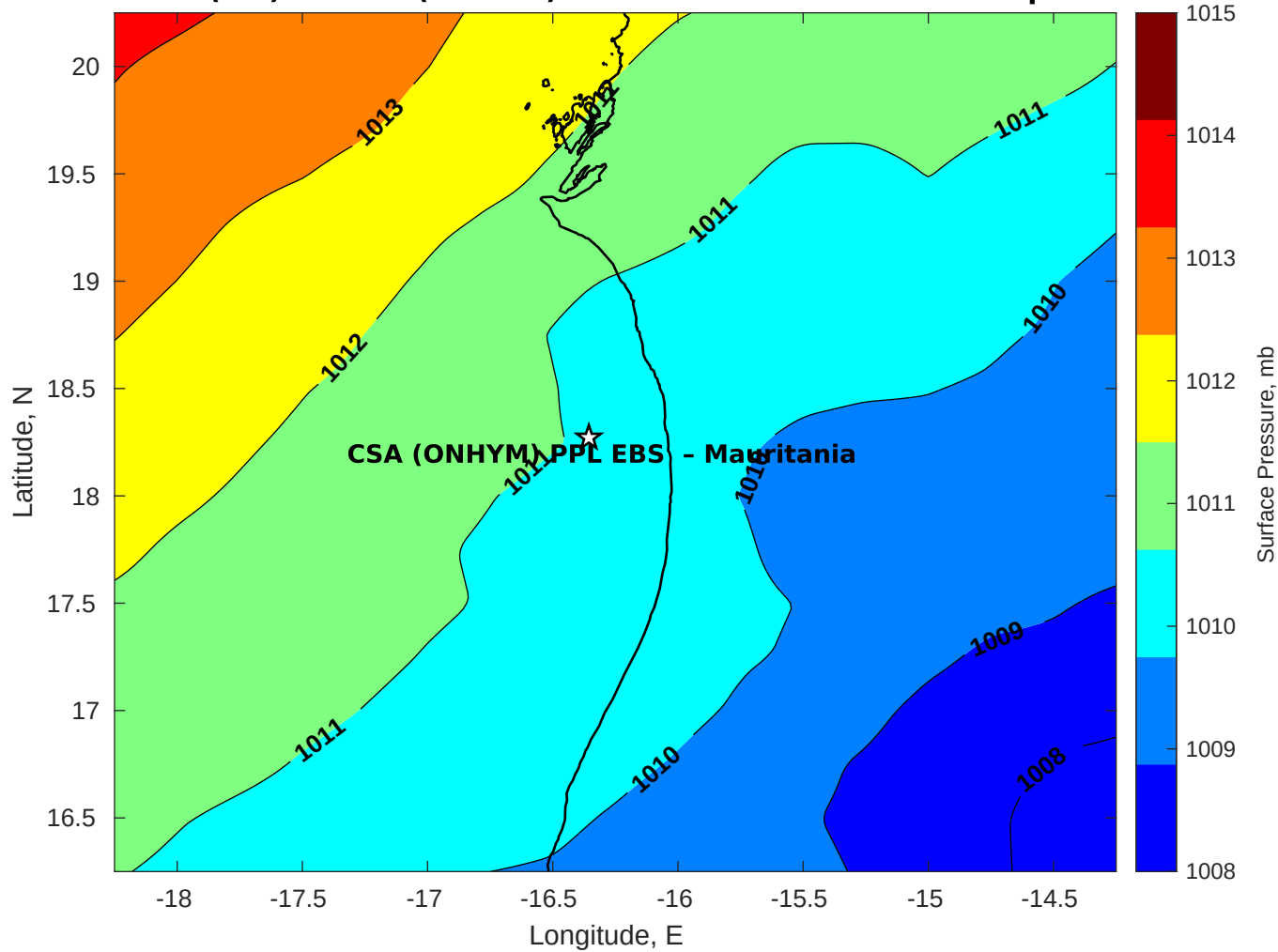
Surface Pressure (mb) for CSA (ONHYM) PPL EBS - Mauritania at 24-Apr-2025 00:00:00
