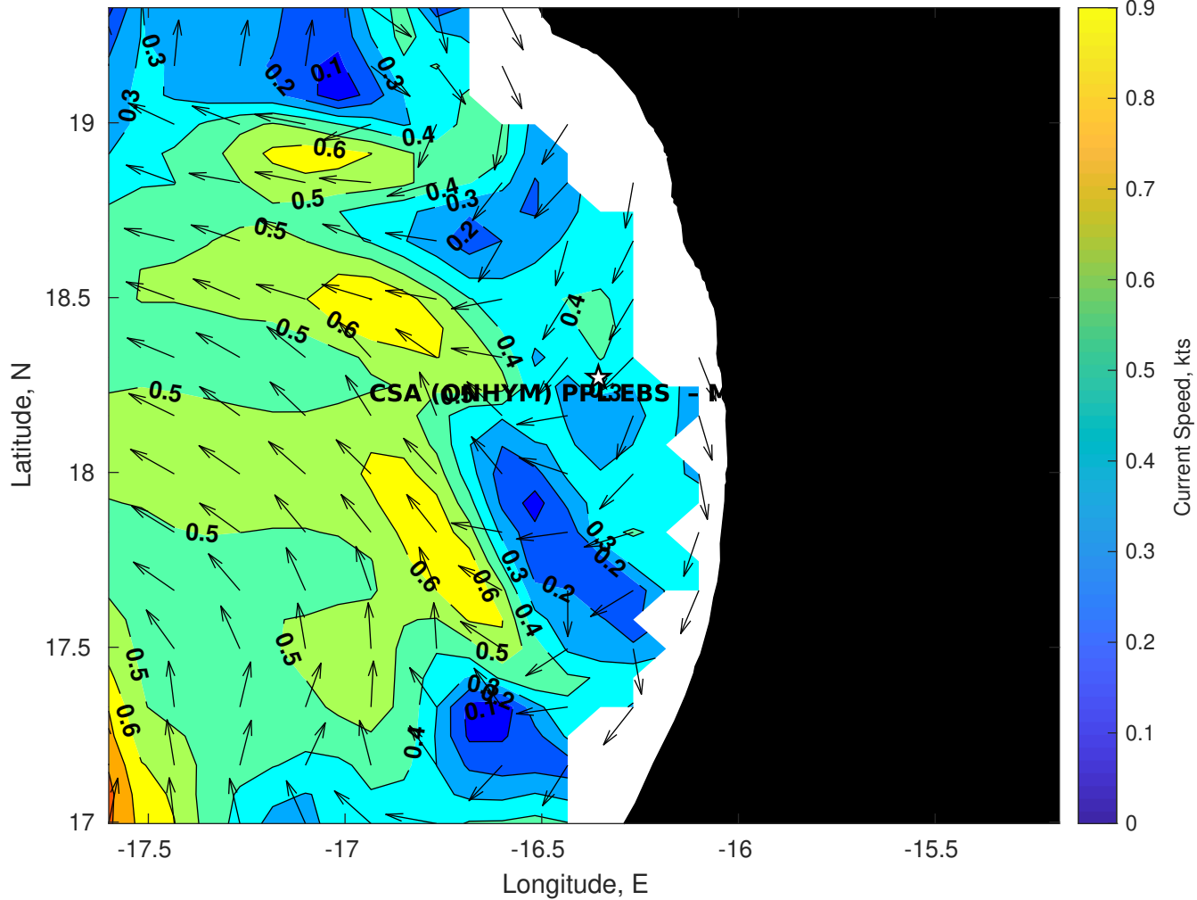
Surface Currents for CSA (ONHYM) PPL EBS - Mauritania at 22-Apr-2025 00:00:00
