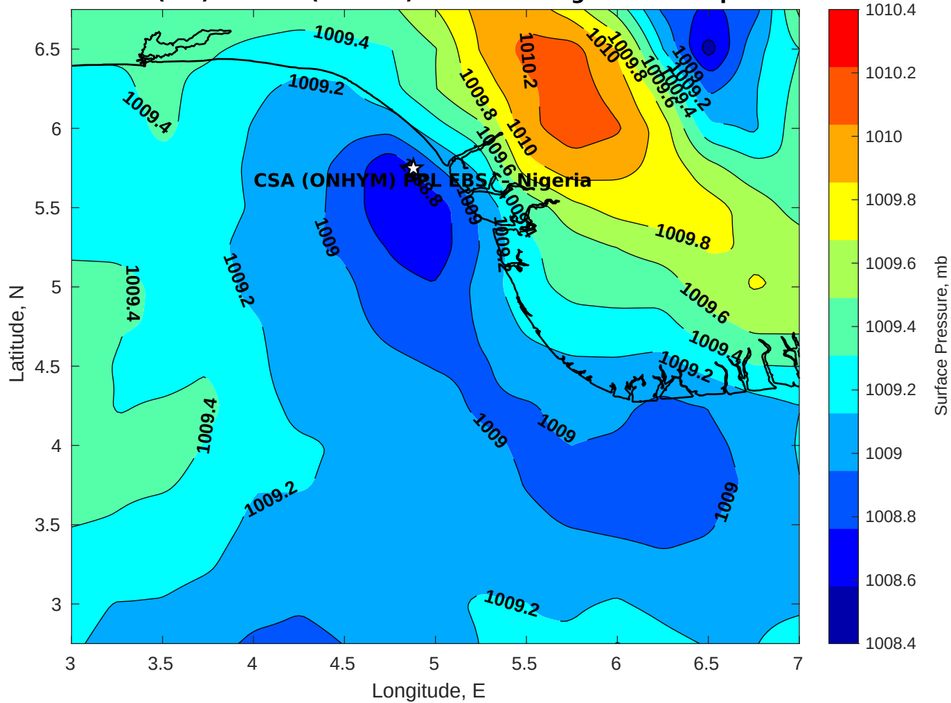
Surface Pressure (mb) for CSA (ONHYM) PPL EBS - Nigeria at 23-Apr-2025 00:00:00
