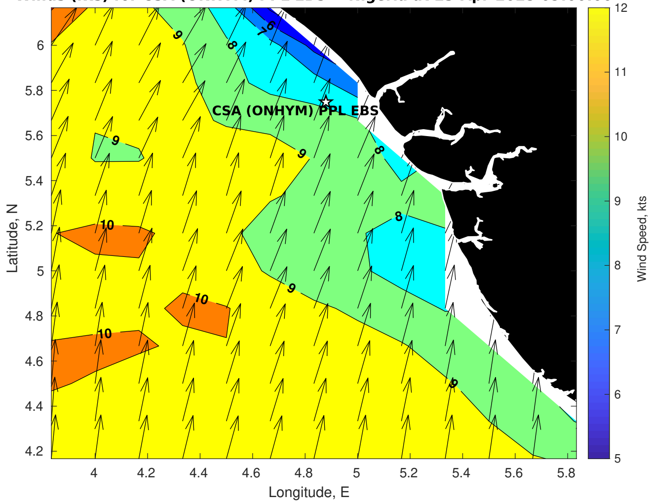
Winds (kts) for CSA (ONHYM) PPL EBS - Nigeria at 23-Apr-2025 09:00:00
