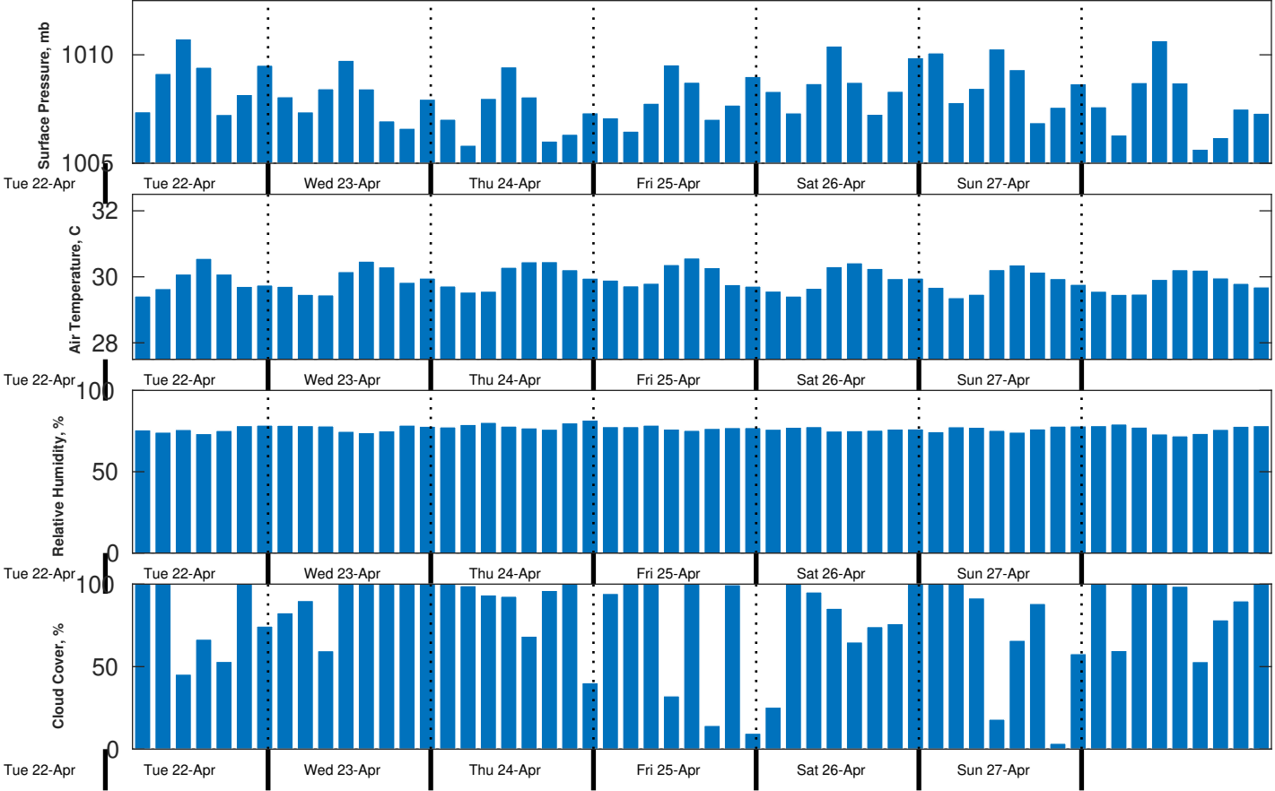
Met Forecast for CSA (ONHYM) PPL EBS - Nigeria from 23-Apr-2025 00:00:00 to 30-Apr-2025 00:00:00
