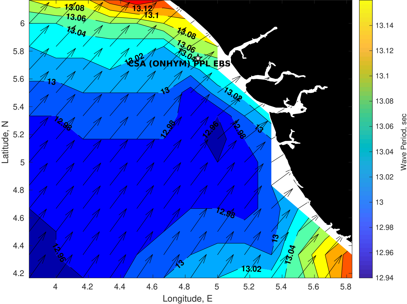
Wave Period (sec) for CSA (ONHYM) PPL EBS - Nigeria at 23-Apr-2025 09:00:00
