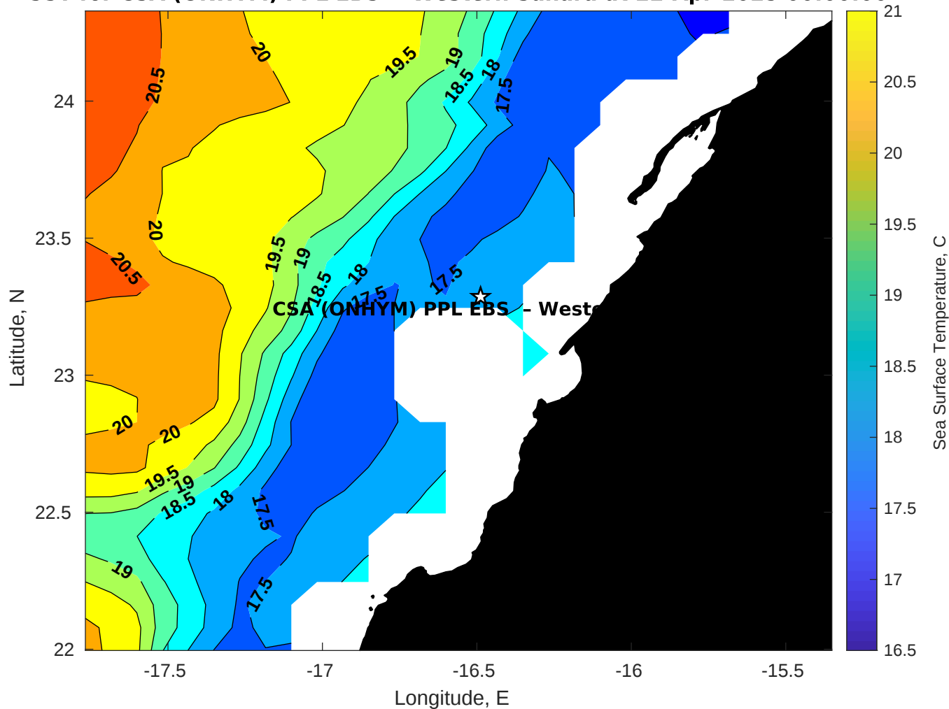
SST for CSA (ONHYM) PPL EBS - Western Sahara at 22-Apr-2025 00:00:00
