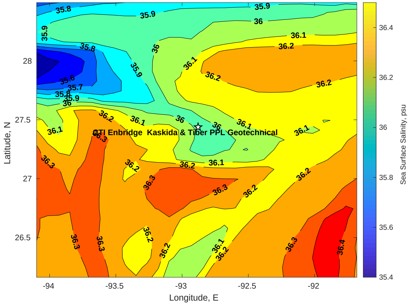
Surface Salinity for CTI Enbridge Kaskida & Tiber PPL Geotechnical at 22-Apr-2025 00:00:00
