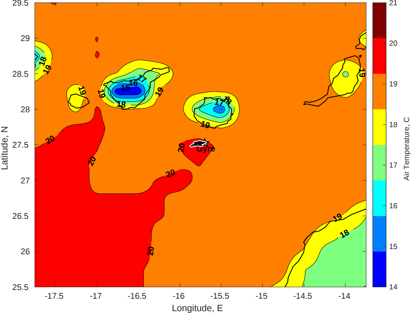
Air Temperature (C) for Gyre at 23-Apr-2025
