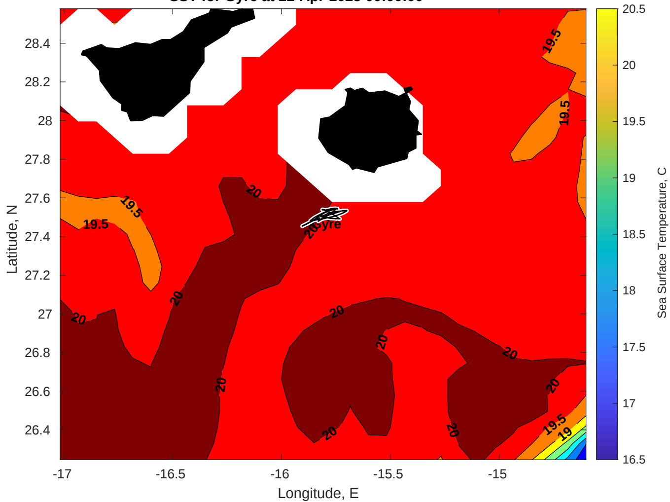
SST for Gyre at 22-Apr-2025 00:00:00
