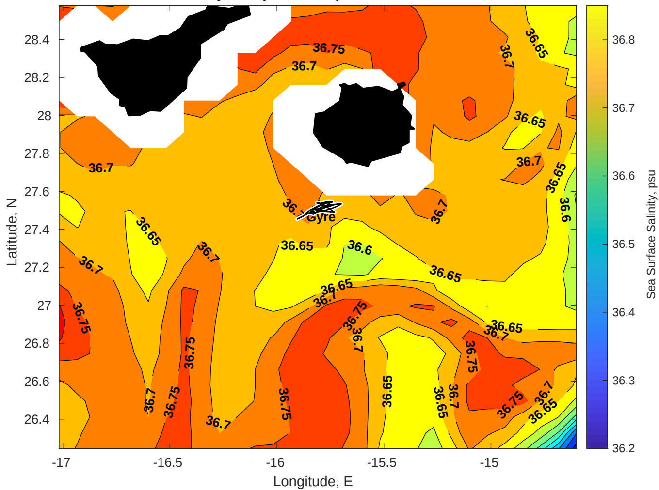
Surface Salinity for Gyre at 22-Apr-2025 00:00:00
