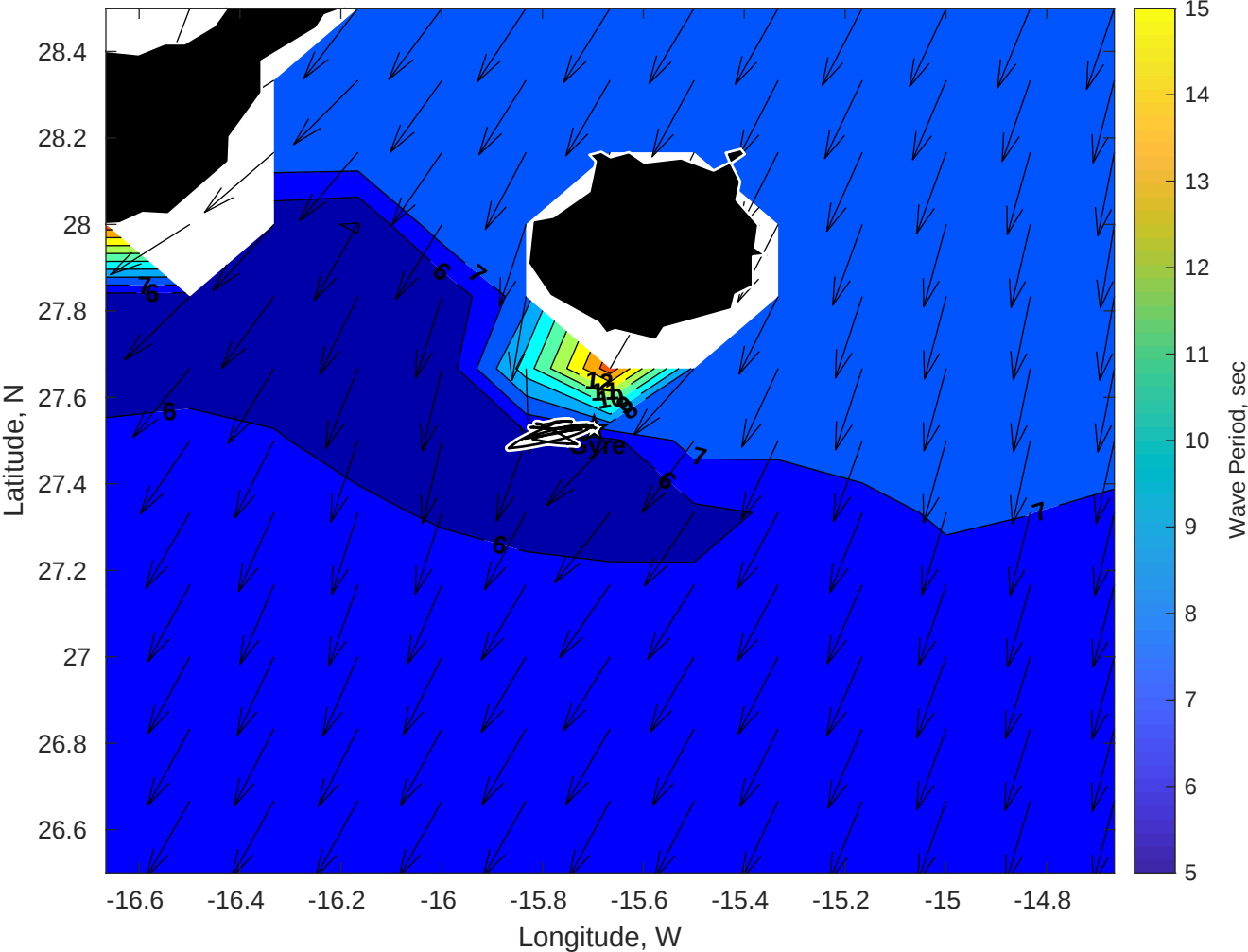
Wave Period (sec) for Gyre at 23-Apr-2025 09:00:00
