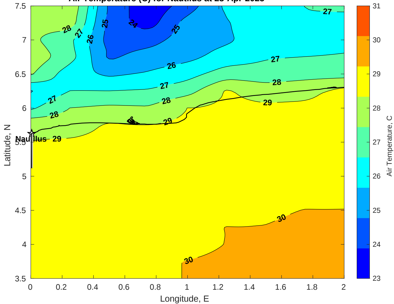
Air Temperature (C) for Nautilus at 23-Apr-2025
