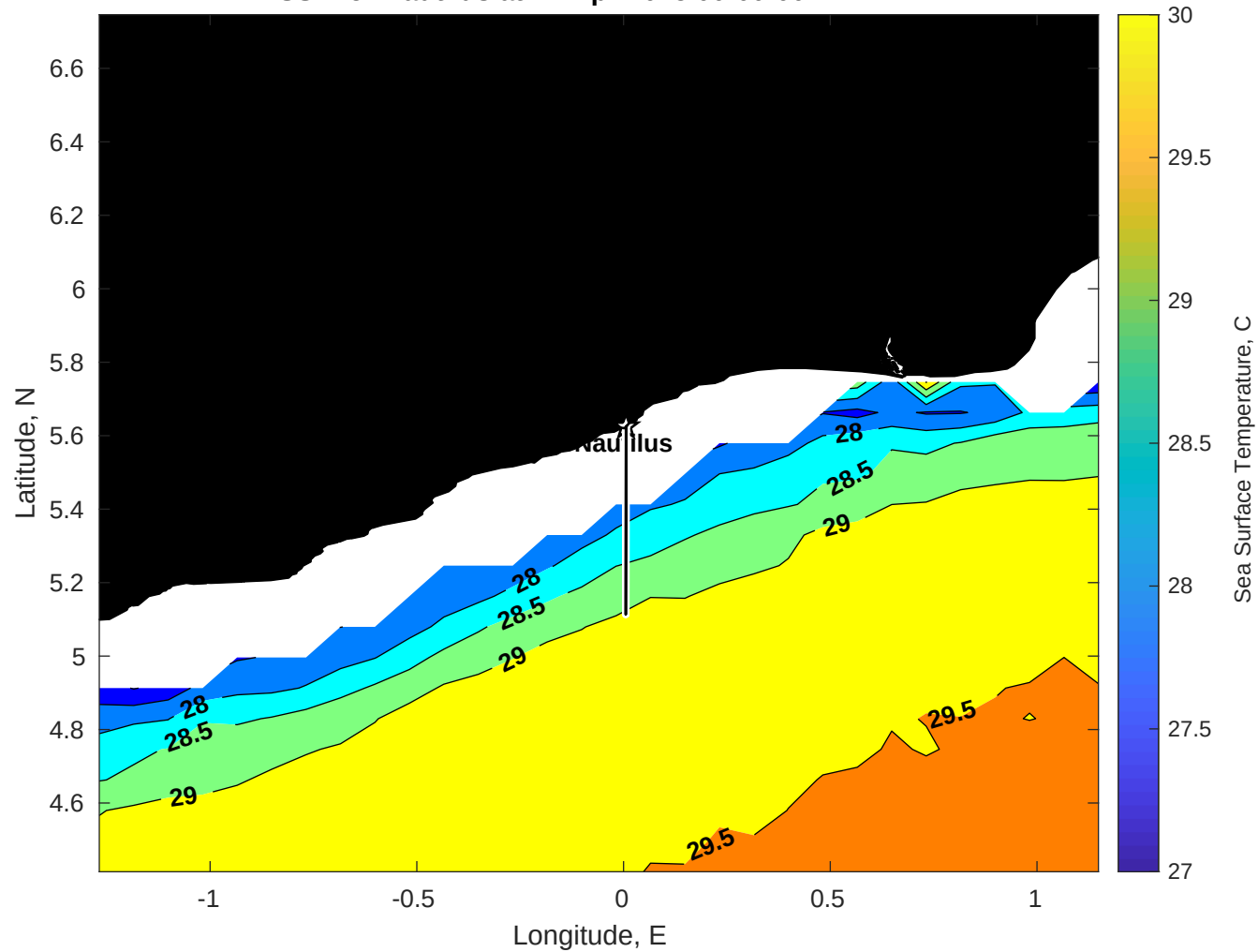
SST for Nautilus at 22-Apr-2025 00:00:00
