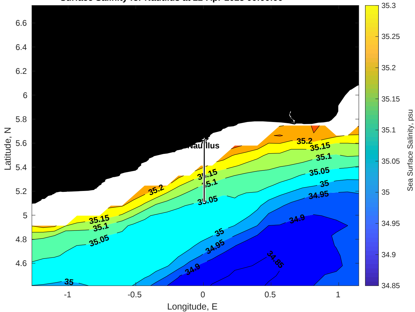
Surface Salinity for Nautilus at 22-Apr-2025 00:00:00
