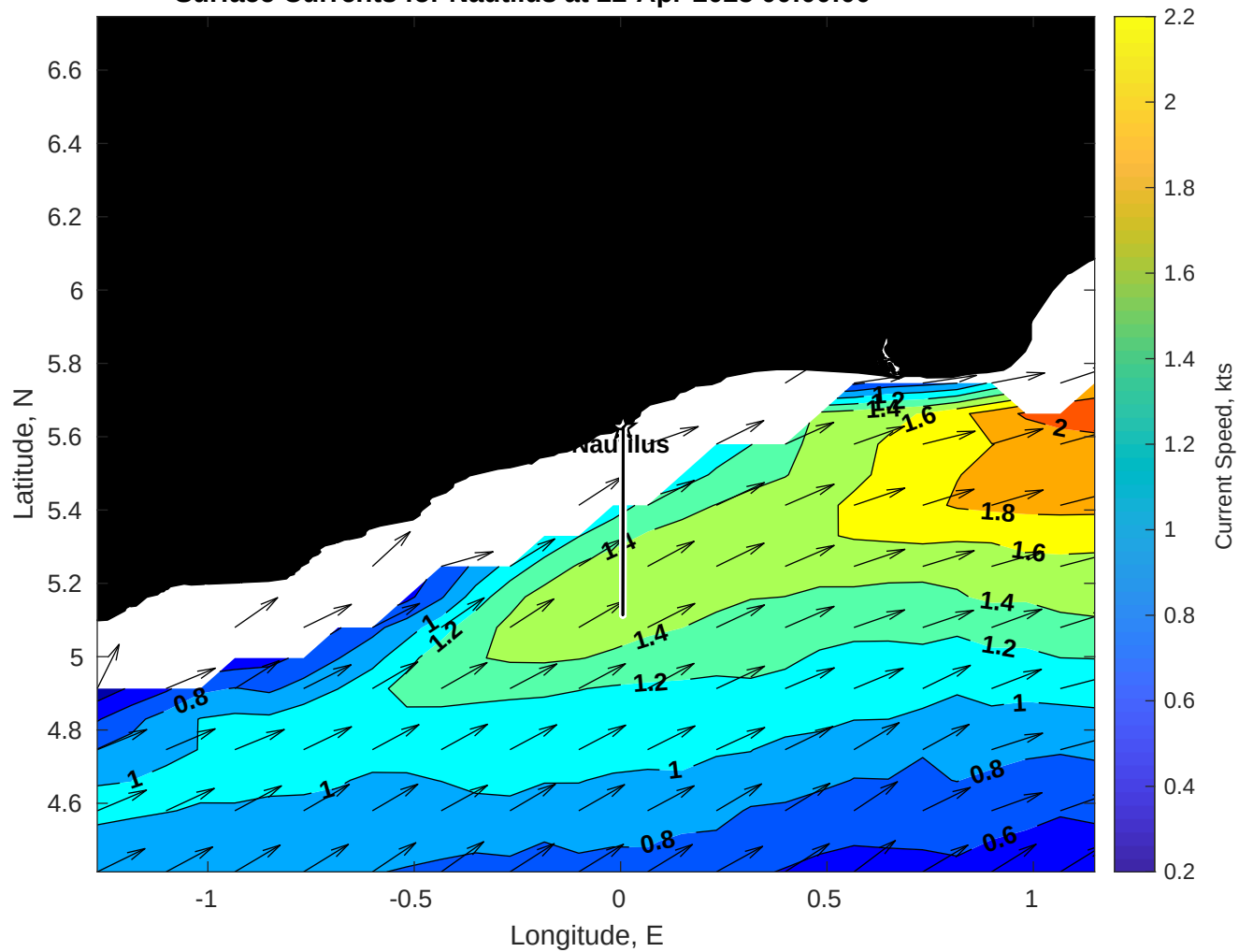
Surface Currents for Nautilus at 22-Apr-2025 00:00:00
