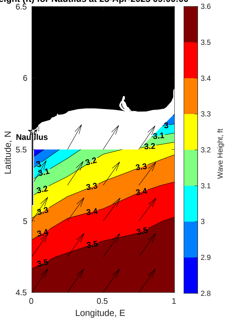
Wave Height (ft) for Nautilus at 23-Apr-2025 09:00:00
