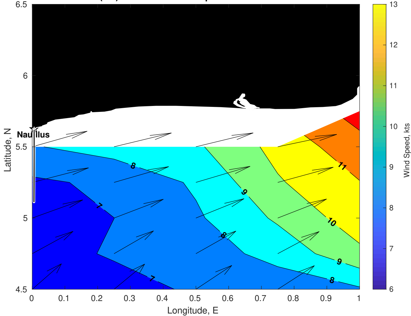
Winds (kts) for Nautilus at 23-Apr-2025 09:00:00
