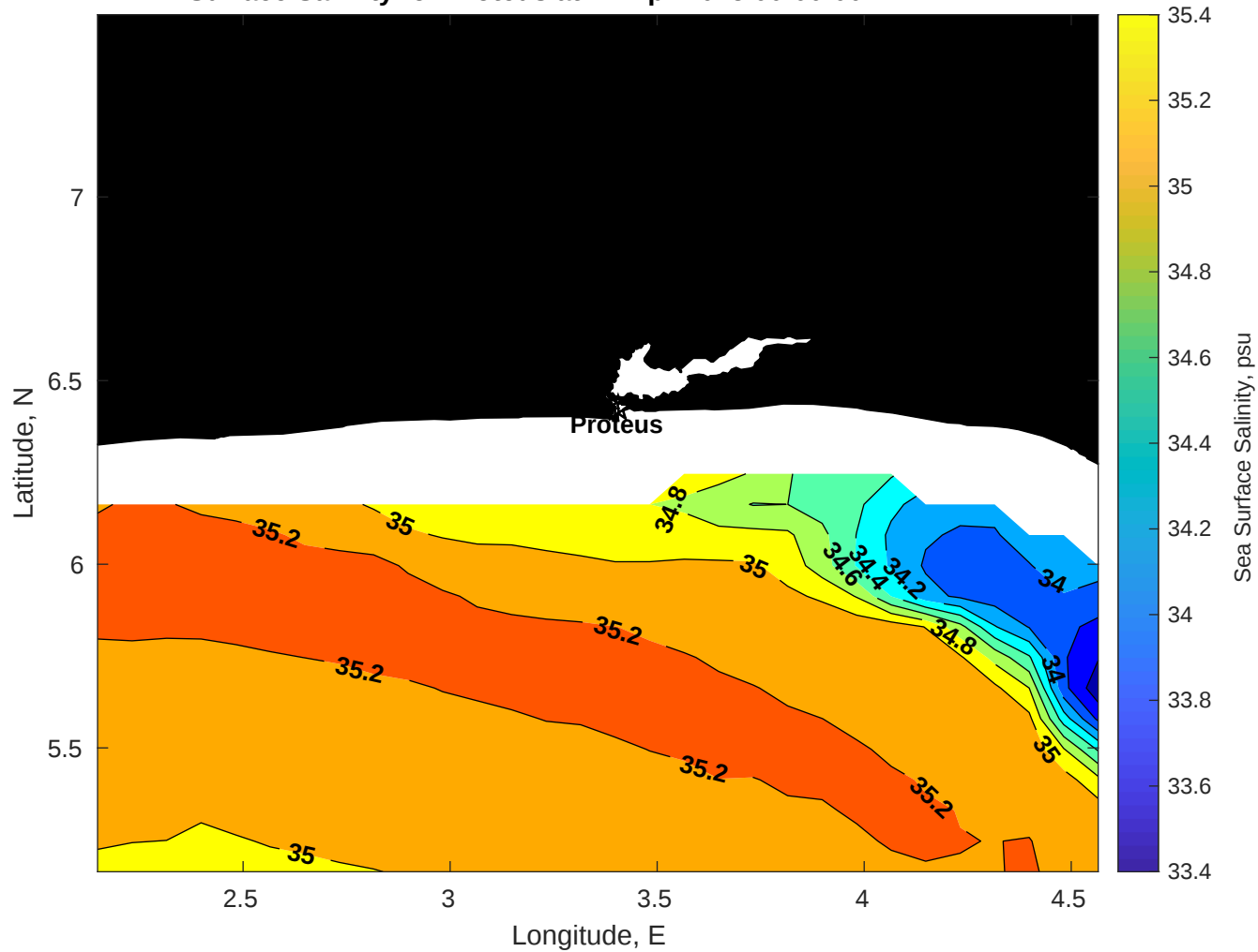
Surface Salinity for Proteus at 22-Apr-2025 00:00:00
