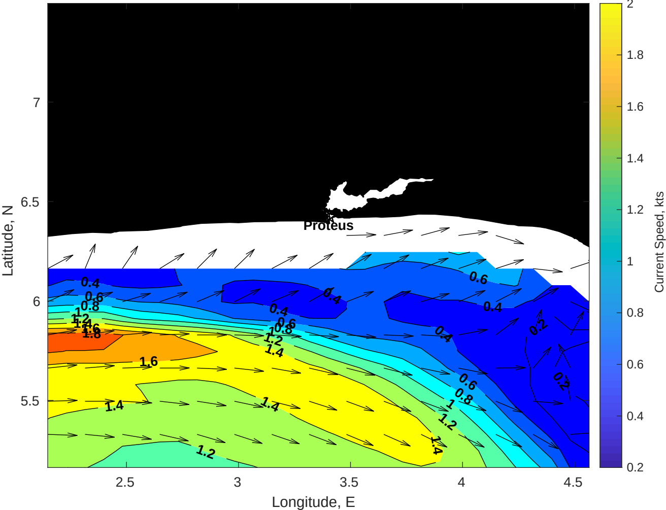
Surface Currents for Proteus at 22-Apr-2025 00:00:00
