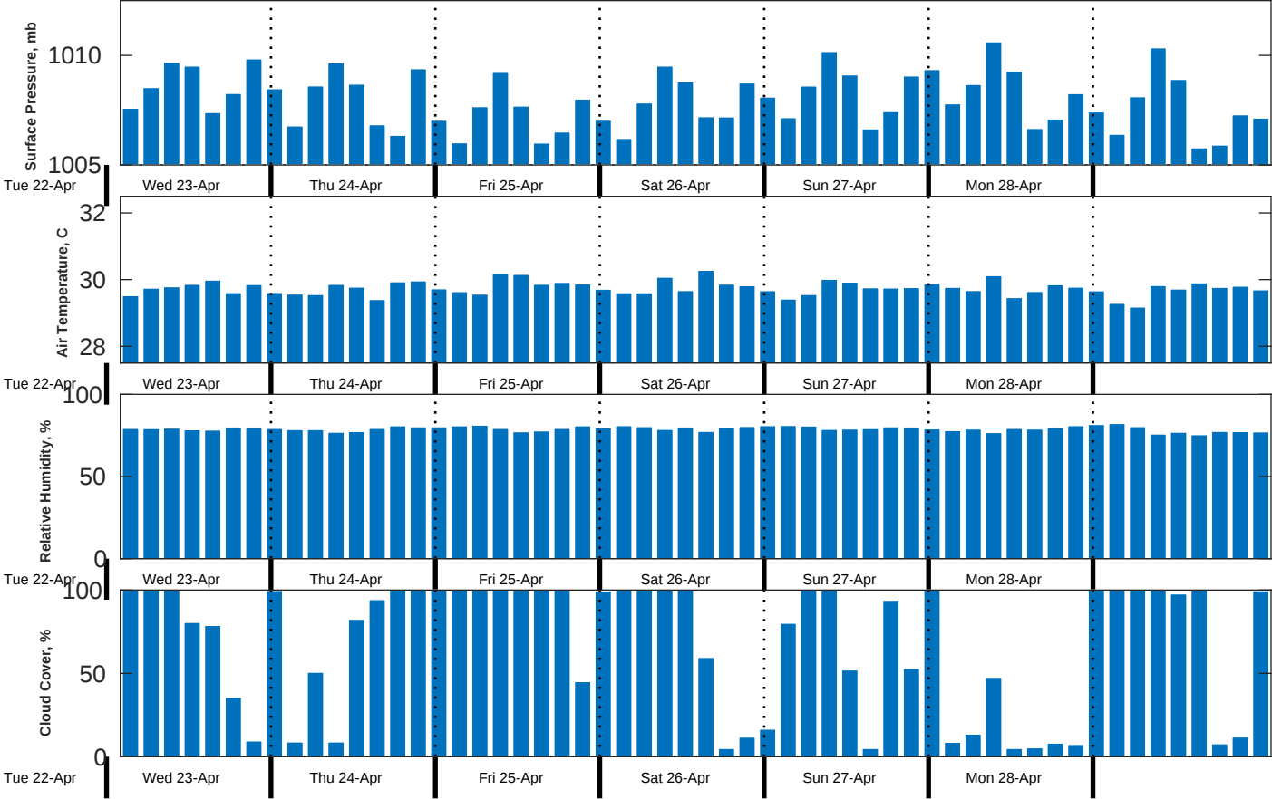
Met Forecast for Proteus from 23-Apr-2025 00:00:00 to 30-Apr-2025 00:00:00
